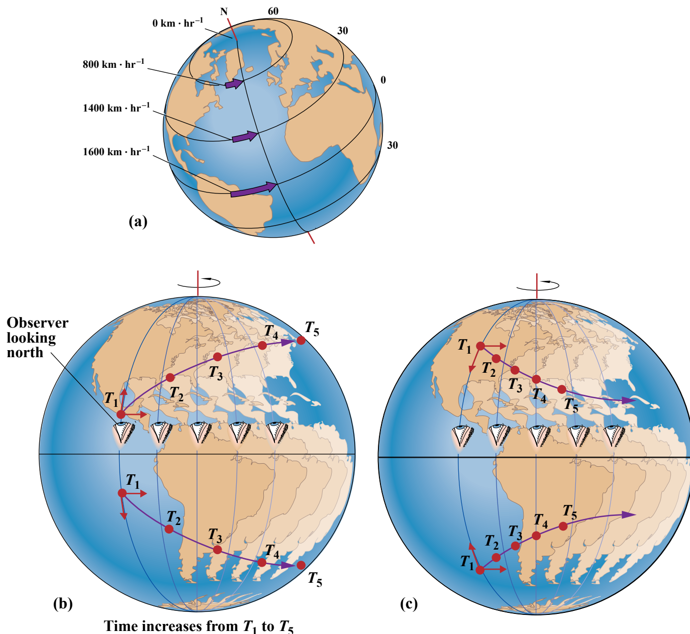
FIGURE CC12-9. (a) The orbital velocity due to the Earth's rotation of points on the Earth's surface decreases as latitude increases. (b) If an object is started in motion directly toward the pole in either hemisphere, it moves progressively into latitudes in which the Earth's surface is moving more slowly in its rotational orbit. However, if the object is moving freely (that is, if it is not attached by strong frictional forces to the solid Earth), it retains the orbital velocity that it had when it was started in motion. Thus, in addition to its motion to the north (or south in the Southern Hemisphere), the object continues to move to the east at its original orbital velocity and progressively moves ahead of the latitude from which it was set in motion. To an observer moving with the Earth's surface, the result is an apparent deflection in the path of the object, to the right in the Northern Hemisphere and to the left in the Southern Hemisphere. (c) If an object is started in motion directly toward the equator in either hemisphere, it moves progressively into latitudes in which the Earth's surface is moving more quickly in its rotational orbit. Thus, in addition to its motion to the south (or north in the Southern Hemisphere), it continues to move to the east at its original orbital velocity and progressively falls behind the latitude from which it was set in motion. The apparent deflection of the path of the object is, once again, to the right in the Northern Hemisphere and to the left in the Southern Hemisphere.
