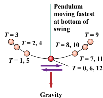
(b) Pendulum slows as it swings upwards.
