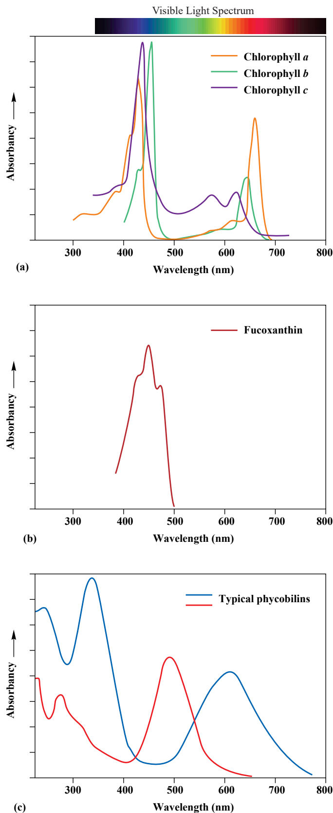
FIGURE CC14-1. Absorption spectra of photosynthetic pigments. (a) Chlorophylls a , b , and c . (b) Fucoxanthin (a typical xanthophyll). (c) Typical phycobilins. Note that the other pigments absorb energy in parts of the spectrum that are not absorbed efficiently by chlorophyll a .
