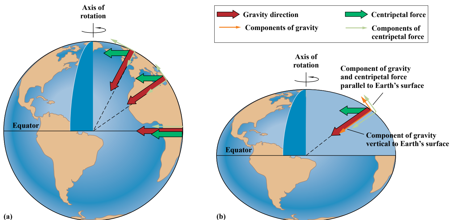
FIGURE CC12-7. (a) If the Earth were exactly spherical, there would be no component of gravity parallel to the Earth's surface at any latitude. However, to keep an object in orbit at the Earth's surface, there would have to be a component of a centripetal force parallel to the Earth's surface, everywhere except at the equator. Because there would be no gravitational force component to provide this component of centripetal force, an object anywhere on the Earth's surface except at the equator would move into a wider orbit (in which the required centripetal force was lower). Thus, the object would slide toward the equator. (b) In response to the force imbalance that would be created if the Earth were spherical, the Earth and all other planets that were at one time totally molten or gaseous were not formed as perfect spheres. Instead, the Earth is an oblate spheroid, a squashed spheroid shape, as shown (but much exaggerated) in the figure. Because the Earth is an oblate spheroid, gravity does not act exactly perpendicular to the Earth's surface, except at the equator and poles. Consequently, at all points other than these, there is a small component of gravity parallel to the Earth's surface that balances the required centripetal force for an object at that point.
