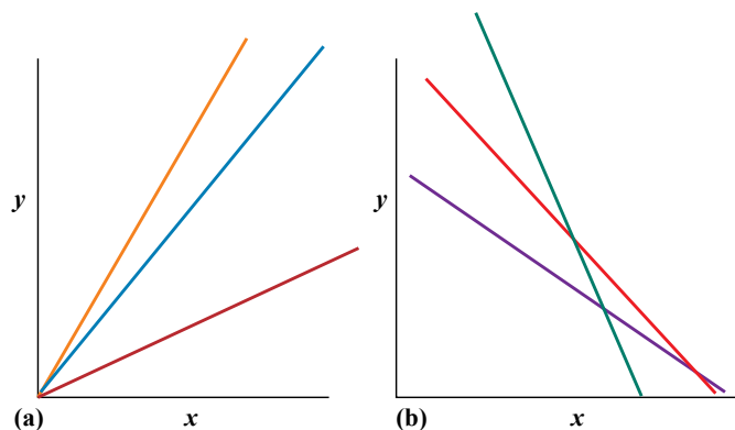
FIGURE CC11-1. Linear relationships can be depicted by the straight line on a graph that plots one variable ( x ) against another ( y ). The value of one variable may (a) increase with an increase in the other variable, or (b) decrease with an increase in the other variable.
