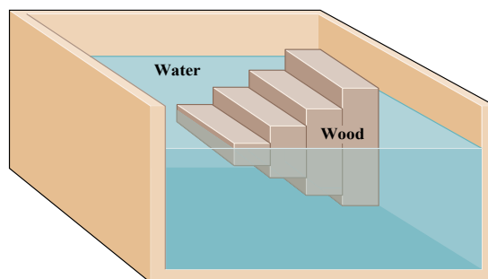
FIGURE CC2-1. Archimedes' principle determines how much of a floating solid's volume is below the surface. The solid floats at a depth such that the weight of the volume of water or other fluid that it displaces (that is, the volume of the part of the solid that is below the water or fluid surface level) equals the total weight of the solid. (a) Lower-density materials will float higher than higher-density materials. (b) Adding weight to a floating, low-density solid increases its mass and causes it to float lower and thus displace more water. The volume of water displaced will have a weight that is equal to the total weight of the floating solid plus the added weight that it supports.
