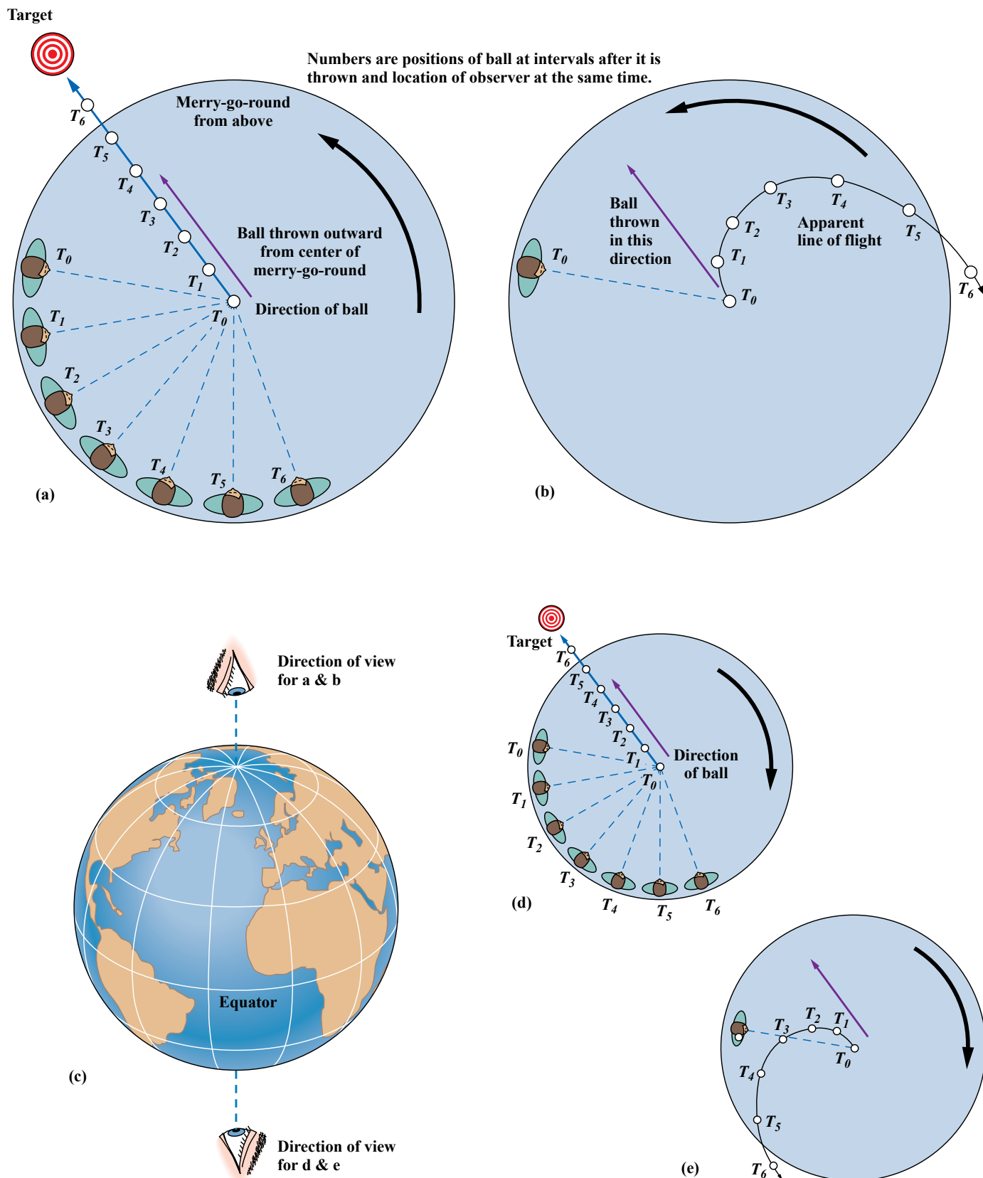
FIGURE CC12-1. (a) A ball thrown outward toward a target from the center of rotation of a merry-go-round has zero orbital velocity due to the merry-go-round's rotation, and will travel outward in a straight line (compared to the ground) to hit the target. However, an observer sitting away from the axis of rotation moves around with the merry-go-round such that the observer's angle of vision to the ball and target changes. (b) If the observer is not aware of the merry-go-round rotation (just as we are not aware of the Earth's rotation), the observer will see the ball appear to move in a circular path, curving to the right. To observe this phenomenon, rotate part (a) to place the observer at the observing location in part (b) for each of the time intervals T_1 , T_2 , and so on. (c) Looking down on the merry-go-round depicted in parts (a) and (b) is equivalent to looking down on the Earth from above the North Pole. If we were to look down from above the South Pole, the merry-go-round would appear to rotate clockwise instead of counterclockwise. (d) If the merry-go-round rotates clockwise (the equivalent of the Southern Hemisphere), the ball still moves in a straight line. However, (e) the apparent deflection is in the opposite direction, and the observer sees the ball curve to the left.
