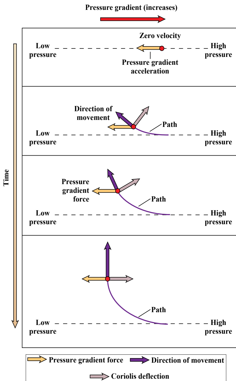
FIGURE CC13-1. When a current is initiated on a horizontal pressure gradient, the initial direction of motion is directly down the gradient. However, as it moves, the water mass is deflected by the Coriolis effect. It accelerates and is deflected until it flows directly across the pressure gradient, and the pressure gradient force is balanced by the Coriolis deflection. This is a “geostrophic” current. If the pressure gradient is steeper, the acceleration is greater, and the geostrophic current is faster, but it is still balanced by the greater Coriolis deflection associated with the higher speed.
