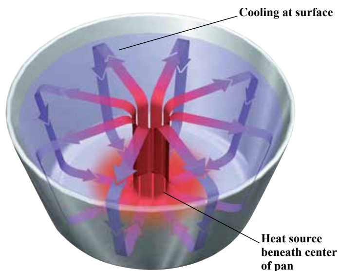
FIGURE CC3-1. In a saucepan heated at the center of its bottom, water will establish a circulation in which heated water rises to the surface, spreads toward the pan’s sides, cools, and then sinks back to the bottom. This toroid-shaped convection cell is established because the water’s density decreases when it is heated and increases when it is cooled. The idealized toroidal convection cell depicted would, in practice, normally be distorted because saucepans are usually heated across their entire base, not just at the center, and by turbulence in the flow patterns caused by variations in the rate of heating and cooling.
