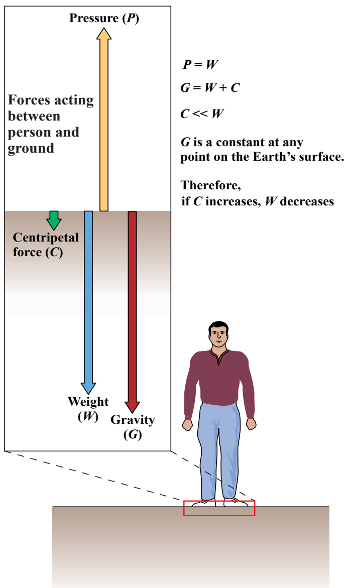
FIGURE CC12-8. There is a balance between the vertical components of gravity (which is invariable at any given location on the Earth), centripetal force, and the Earth's pressure gradient for objects moving over Earth's surface. The pressure gradient force is equal to the object's weight. The pressure gradient force and the object's weight must be very slightly smaller than the gravitational force because the gravitational force must provide the required centripetal force to maintain the object in its orbit with the rotating Earth. Thus, the object's weight equals the gravitational force minus the very much smaller centripetal force. The magnitude of the centripetal force has been greatly exaggerated in this figure.
