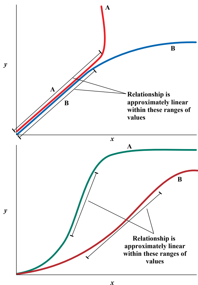
FIGURE CC11-2. Nonlinear relationships can be identified by the curvature of a graph that plots one variable ( x ) against another ( y ). Although the curvature can be complex, there is often a range of two values within which the relationship is approximately linear.
