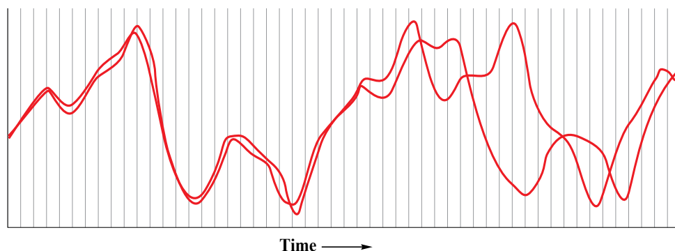
FIGURE CC11-4. These two plot lines depict the results obtained from the same nonlinear mathematical model that simulates weather patterns. The only difference between the two model runs is that the starting-point data were rounded to a smaller number of decimal places for one model run than for the other. The patterns grow farther and farther apart until they lose any resemblance to each other. Many natural systems show this sensitive dependence on initial conditions. As a result, it is impossible to measure and model such systems well enough to predict their precise future behaviors.
