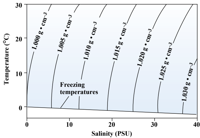
FIGURE CC6-1. The relationships among salinity, temperature, and density are complex. Generally, density increases as temperature decreases or as salinity increases. This figure is reproduced with additional information in Chapter 5 ( Fig. 5-13a ).
