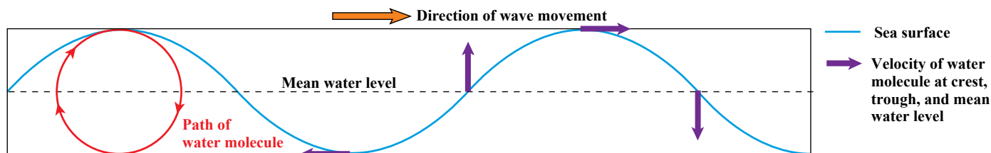
FIGURE 9-3. In a progressive wave, water at the crest is moving forward but has no vertical velocity. After the crest passes, the forward velocity slows, and vertical velocity increases until, halfway between crest and trough, the velocity is entirely vertical. As the wave continues forward, the vertical velocity is slowed, and the water gains velocity in the backward direction. At the trough, the vertical velocity is zero, and the backward velocity is at a maximum. The waveform moves forward, but each particle of water moves in a circular orbit whose diameter equals the wave height (for water at the surface) and returns to its starting point after each wave. You can see this for yourself if you push down on a water bed. The wave travels across the bed, but the plastic “surface layer” returns to its original location after the wave has passed.
