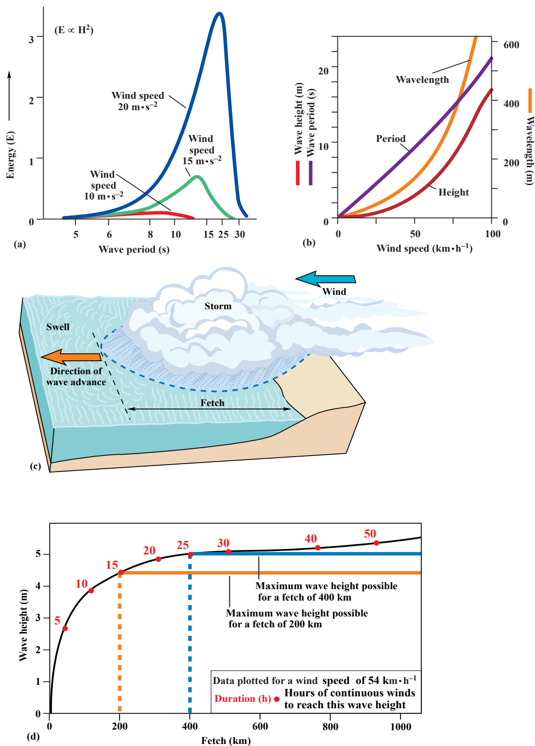
FIGURE 9-7. Relationships between wind speed, fetch, the length of time over which the wind blows, and the characteristics of the waves that are formed. (a) Strong (higher-speed) winds produce storms with greater total wave energy, and this energy is stored in waves of longer periods. (b) Strong winds also produce waves that have longer wavelengths and greater wave heights, provided that the winds blow long enough and have sufficient fetch. (c) The fetch is the distance over which the winds blow across the water to create waves. Fetch can be limited by the presence of a coastline or, where the storm is completely over water, by the dimensions of the storm itself. (d) The maximum wave height that can be reached is limited by the fetch, and this maximum wave height is reached only if the winds blow for a sufficiently long time.
