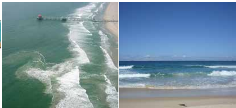
FIGURE 9-23. (a) Rip currents are fast, narrow currents that return water offshore after it has been transported toward the beach that form at intervals along a beach. (b) Rip currents are sometimes visible as foam or discoloration of the water caused by sediments suspended by turbulence in the swiftly moving current. This type of rip current is not in a fixed location on the beach and may appear quickly and dissipate just as quickly. (c) A more permanent type of rip current may form where water runs through a channel on the seafloor. This type can often be seen as a gap in the breaking crests of the waves.
