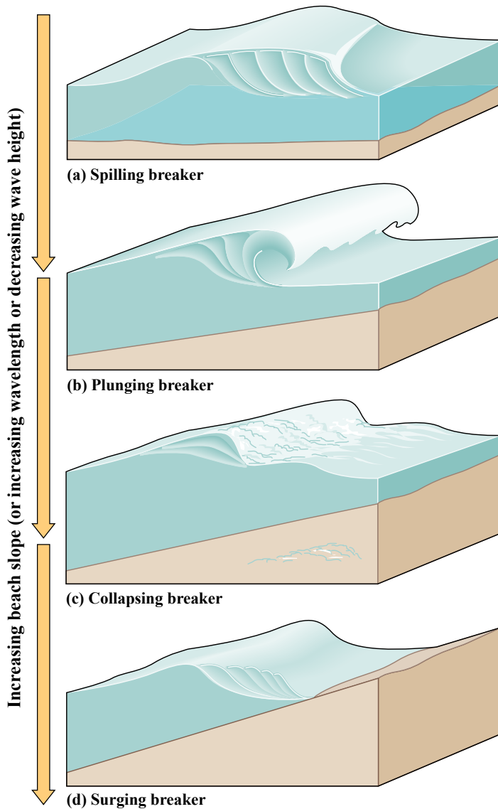
FIGURE 9-20. Breaking waves. (a) The peak of a spilling breaker becomes oversteepened, and it breaks by spilling water from the crest down the front face of the wave. (b) The peak of a plunging breaker travels fast enough to outrun the rest of the wave, and the crest curls over and smashes down on the front of the wave. (c) The base of the front side of a collapsing breaker becomes unstable before the crest, and the front face of the wave collapses. (d) A surging breaker never really breaks. The front face of the wave simply surges up and down on the beach, and the wave energy is partially reflected back out to sea.
