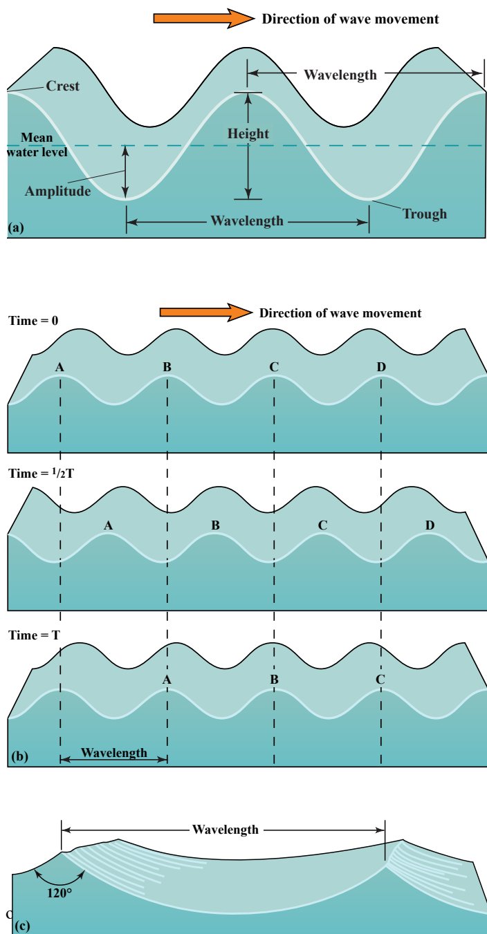
FIGURE 9-2. (a) All waves can be characterized by the presence of a crest and a trough, and by their wavelength ( L ) and wave height. (b) Progressive waves travel over the ocean surface at a speed that can be characterized by their period ( T ) or their frequency ( f ), which is the inverse of the period. Most progressive waves are smooth sine waves with rounded crests and troughs. (c) As waves are built by the wind, they develop a pointed crest and become trochoidal in shape.
