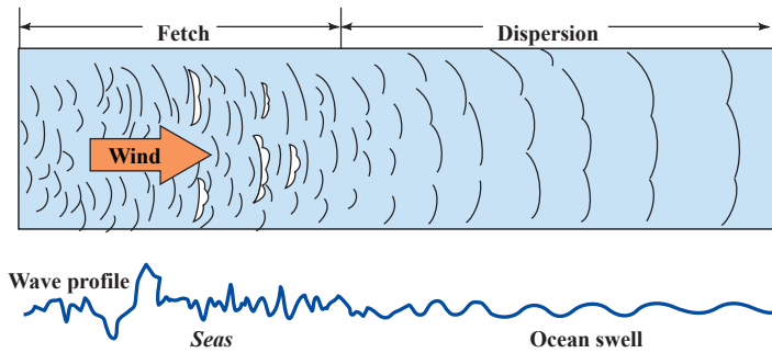
FIGURE 9-15. Within the fetch of a storm, the waves are irregular because they are the sum of many separate waves of different wavelengths, as shown in Figure 9-12. Long-wavelength waves move faster than shorter-wavelength waves, such that, as waves move away from the storm, the long-wavelength waves move ahead of the shorter-wavelength waves. This sorting of the waves by wavelengths is called wave dispersion. Because they are separated by wavelength, the waves appear to become smoother as they travel away from the storm fetch. The greater the distance from the fetch, the greater the difference in the arrival times of waves of two different wavelengths.
