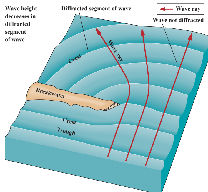
FIGURE 9-22. A wave is diffracted when the wave crest encounters a solid object, such as a breakwater. The part of the wave that passes by the end of the breakwater is bent such that the wave spreads out behind the breakwater.
