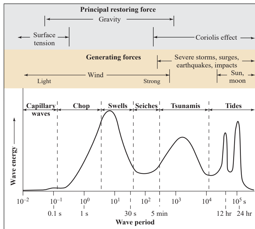
FIGURE 9-5. It is estimated that most of the energy associated with waves in the world’s oceans is contained in wind waves that have periods of between 0.2 and 30 s. However, there is also considerable energy associated with tides (periods of 12 h and above) and, despite their infrequent occurrence, considerable energy is also associated with tsunamis and severe storm waves (periods between about 1 min and 1 h). The smallest waves, capillary waves, are created by winds and restored principally by surface tension. Winds are responsible for creating most waves with periods less than about 15 min, and gravity is responsible for restoring all except the shortest-period capillary waves within this range of periods. Longer waves are formed by earthquakes and tidal forces, and the Coriolis effect is the principal restoring force for the longest waves.
