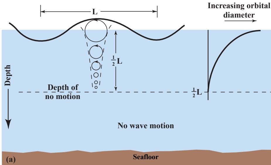
FIGURE 9-10 Orbital motion of water particles beneath waves. (a) The orbits in which individual particles move within a wave decrease in diameter exponentially with increasing depth. The wave motion becomes essentially zero at a depth equal to one-half of the wavelength. (b) The particle orbits are not exactly closed. Instead, each particle moves forward a very small distance (exaggerated in this figure) during each orbit. Therefore, there is a very small net mass transport of water in the direction of the wave.
