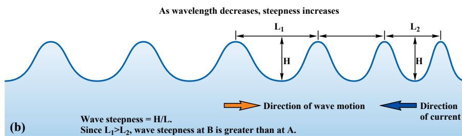
FIGURE 9-8. (a) Waves from around Antarctica travel northward and meet the strong, southward-flowing Agulhas Current. (b) As each wave encounters the current, its forward speed is decreased because the current moves surface water southward, and water particles in each wave are a little farther south after each wave orbit, instead of in their original position. As each wave slows, the following wave that has not yet encountered the current is not slowed, so its crest becomes closer to the crest of the wave preceding it. Hence, wavelength decreases and steepness increases as the figure shows. (c) The tanker World Glory , sinking after breaking its back in waves steepened by the Agulhas Current.
