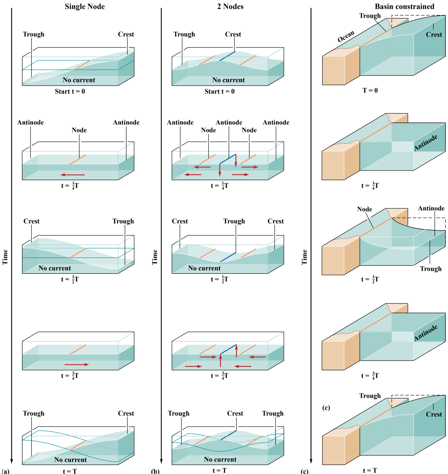
FIGURE 9-25. The motion of water in standing waves. The standing-wave motion is a seesaw oscillation of the surface. Standing waves have one or more nodes (where there is no change in the water surface height but there are oscillating horizontal currents) and one or more antinodes (where there are no currents but the surface oscillates up and down). (a) A standing wave with a single node. (b) A standing wave with two nodes. (c) A standing wave that is essentially a half wave with a node at the basin entrance and only one antinode, at the closed end of the basin.
