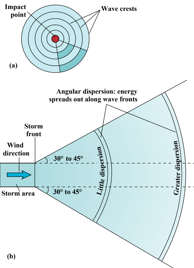
FIGURE 9-9. (a) Waves spread out uniformly in all directions from an impact point, and energy is spread along the increasing length of each wave as it moves away from this point. (b) Waves generated along a storm front travel forward in the direction of the winds in the storm, but they also spread out in a fan shape. This disperses (spreads) the wave energy along a progressively lengthening wave crest with distance from the storm.
