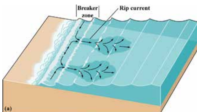
FIGURE 9-23. (a) Rip currents are fast, narrow currents that return water offshore after it has been transported toward the beach that form at intervals along a beach. (b) Rip currents are sometimes visible as foam or discoloration of the water caused by sediments suspended by turbulence in the swiftly moving current. This type of rip current is not in a fixed location on the beach and may appear quickly and dissipate just as quickly. (c) A more permanent type of rip current may form where water runs through a channel on the seafloor. This type can often be seen as a gap in the breaking crests of the waves.
