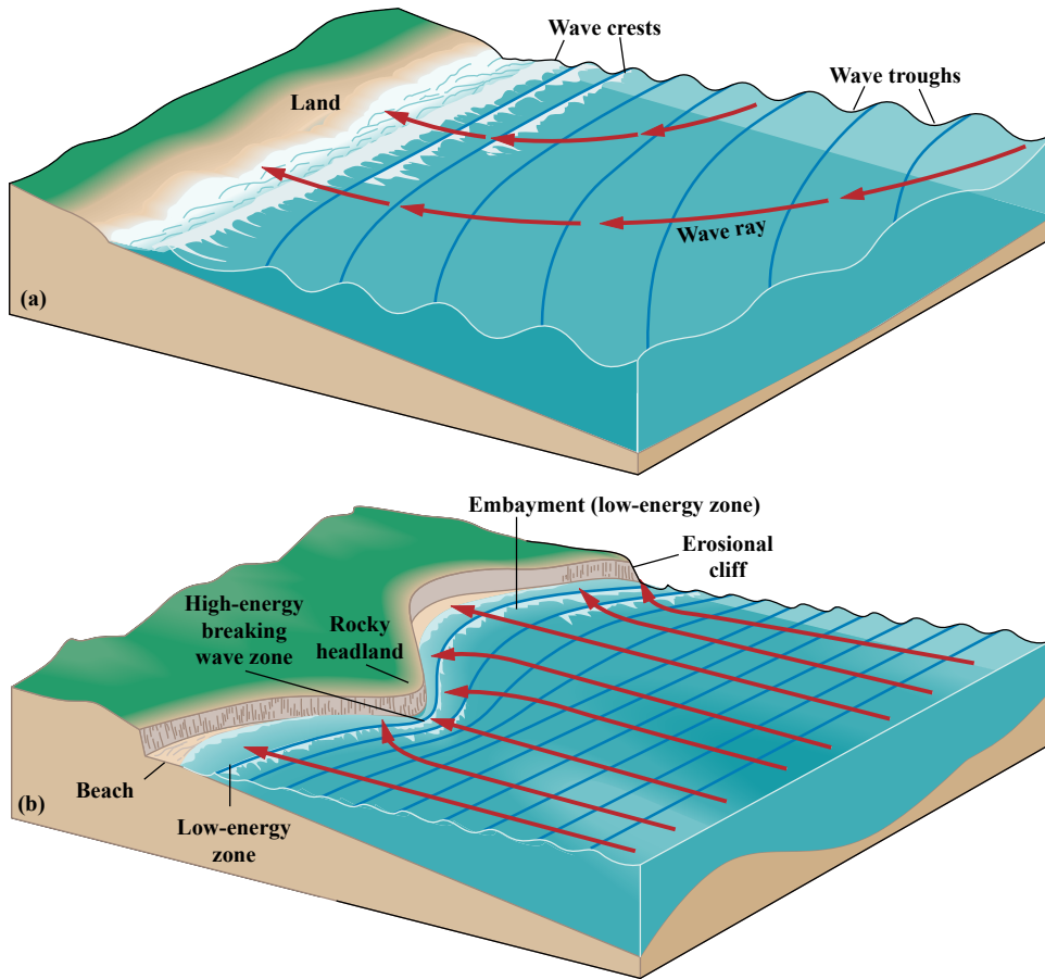
FIGURE 9-18. Wave refraction. (a) Waves generally approach the coastline at an angle. Consequently, part of the wave front reaches shallow water and is slowed before the rest of the wave. It continues to slow as the other parts of the wave move more rapidly toward shore until they, too, are progressively slowed. As a result, the wave front is bent and becomes aligned more closely parallel to the beach. The path followed by any point on the wave crest is called a wave ray. (b) As a wave approaches a bay flanked by headlands whose topography extends onto the offshore seafloor, the first parts of the wave to slow are those over the underwater extensions of the headlands, and the last part to be slowed is that over the deeper water at the center of the bay. Thus, the wave is refracted, and wave energy is concentrated on the headlands and spread out inside the bay. Breaking waves are the strongest at the headlands.
