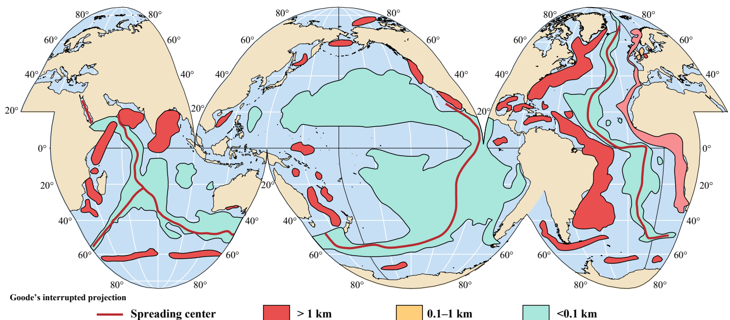
FIGURE 6-17. Thickness of accumulated sediments on the world's oceanic crust.
