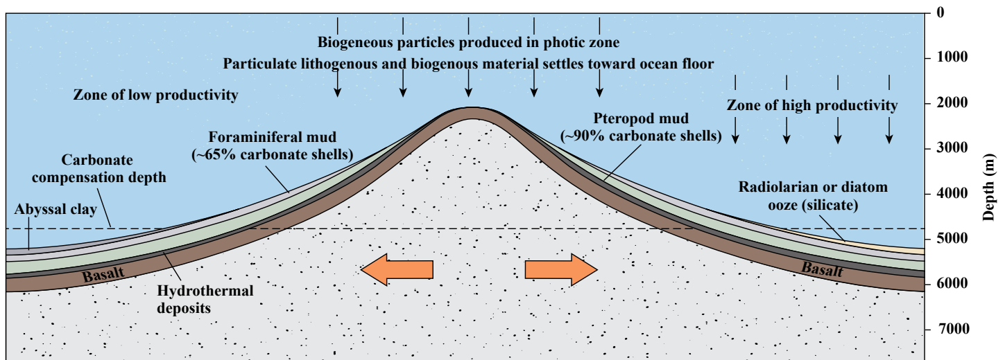
FIGURE 6-11. Idealized depiction of layered sediment accumulation on an actively spreading oceanic ridge. There is a thin, patchy cover of predominantly hydrothermal sediments at the center of the oceanic ridge. On the flanks of the ridge, which are shallower than the carbonate compensation depth (CCD), calcareous sediments dominated by pteropods and foraminifera are deposited. Pteropods dominate the surface sediments only at depths much shallower than the CCD because their shells are made of a more soluble form of calcium carbonate than those of foraminifera. As the new oceanic crust moves away from the spreading center and sinks isostatically, it is covered by layers of hydrothermal sediments, pteropod and foraminiferal oozes, and then siliceous sediments in sequence as the seafloor descends. The siliceous sediments can be either biogenous, if diatomaceous or radiolarian production in the overlying water column is high, or fine-grained lithogenous clays. In the Pacific Ocean, the lithogenous sediments are primarily deep-sea clays because subduction zones prevent inputs of turbidites. In the Atlantic Ocean, they are generally a mixture of deep-sea clays and turbidites.
