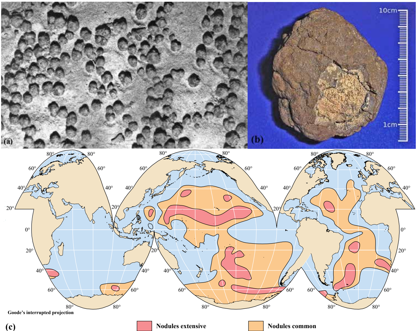
FIGURE 6-12. (a) Manganese nodules cover certain areas of the deep-ocean floor, such as this area of the northeastern Atlantic Ocean. (b) A typical manganese nodule. The nodule is made up of concentric layers. (c) The areas of the greatest density of manganese nodules are on the abyssal floor of the North Pacific Ocean between about 10°N and 20°N and in the central South Pacific Ocean.
