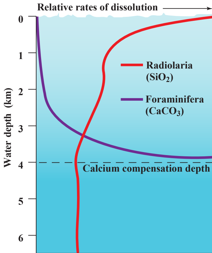
FIGURE 6-10. Changes in the dissolution rate of siliceous shells (radiolaria) and calcareous shells (foraminifera) with depth. Siliceous shells are more soluble in surface layers; calcareous shells are more soluble at greater depth.
