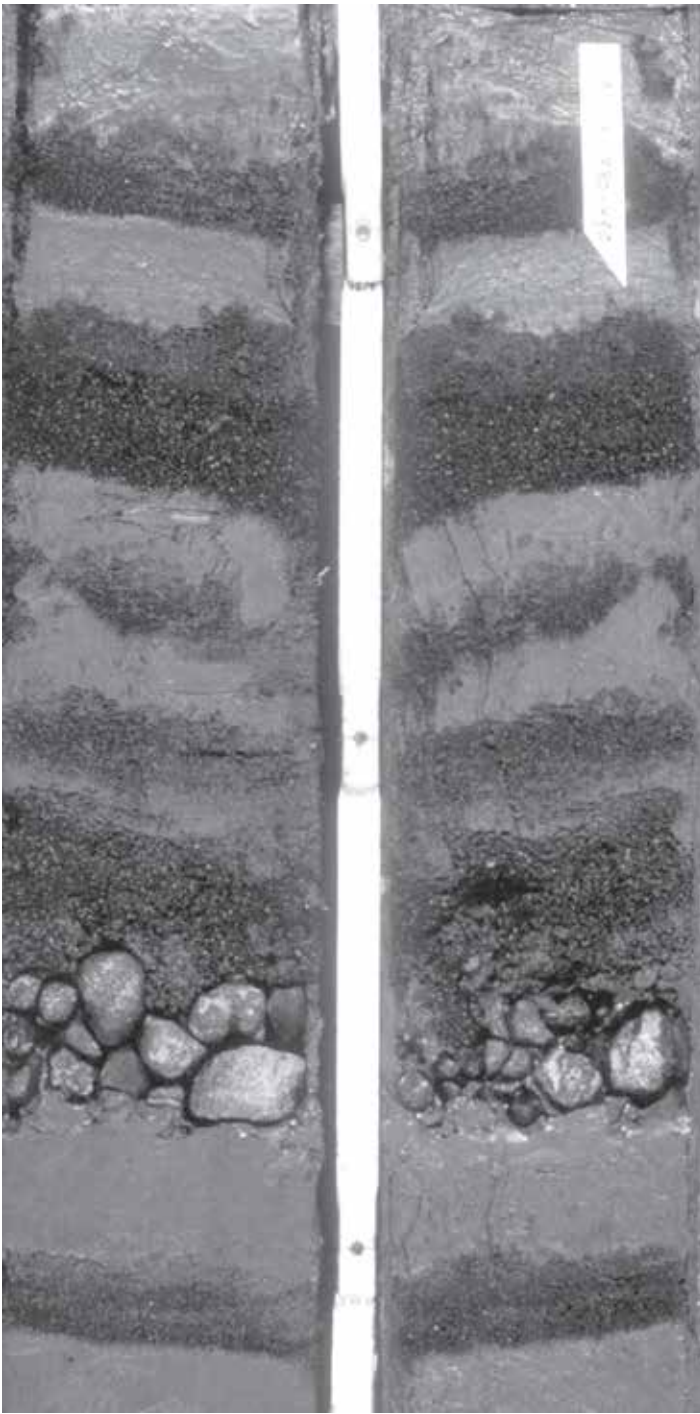
FIGURE 6-14. There are a number of turbidite layers in these cores. Note the sharp change in grain size at the bottom of each turbidite layer and the gradual reduction in grain size above this boundary. The convex shape of the boundaries between layers is due to distortion of the core during the drilling process. Most turbidite layers would not exhibit the very large particles seen at the lower part of some of the turbidite layers. However, these cores are from the Antarctic continental slope, where large particles are carried onto the continental shelf by glaciers.
