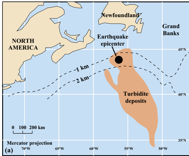
FIGURE 6-15. Submarine cables in the North Atlantic were severed in succession by an earthquake-triggered turbidity current in 1929. (a) The earthquake epicenter was located on the continental slope. Turbidity currents caused by the earthquake spread turbidite sediments across large areas of the deep-sea floor, extending more than 1000 km from the source. (b) The turbidity currents broke several submarine telephone cables at precisely known times. From these data, it was found that the turbidity currents had reached speeds in excess of 70 \text{ km} \cdot \text{h}^{-1} .
