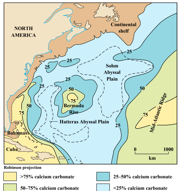
FIGURE 6-13. Calcium carbonate distribution in the sediments of the western North Atlantic. Values are the percentage of calcium carbonate in the sediment. The high percentages of calcium carbonate in the Bahama Banks sediments are due primarily to the dominance of hydrogenous calcium carbonate. In the shallow parts of the Bermuda Rise and the Mid-Atlantic Ridge, lithogenous sediment accumulation rates are low, allowing biogenous carbonate particles to dominate the sediments in these regions.
