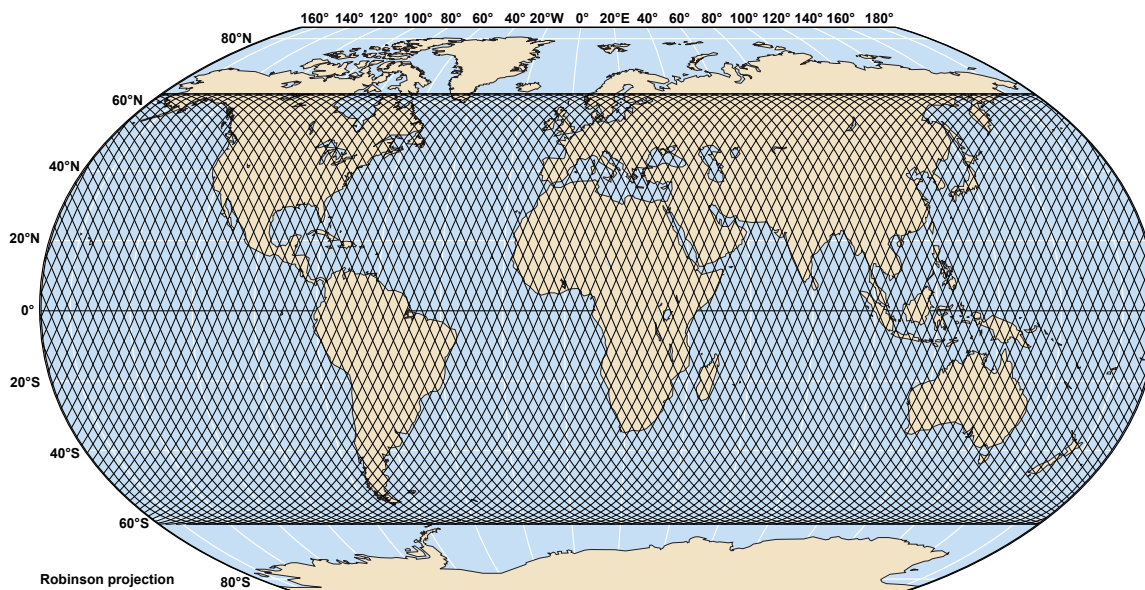
FIGURE 3-27. The TOPEX/Poseidon satellite travels in an orbit 1366 km high and inclined at 66° to the equator, which is typical of satellites used for ocean observations. This orbit allows coverage of 95% of the ice-free oceans every 10 days. The satellite's position is known to within 10 cm from the Earth's center. The network of curved lines on the map schematically illustrates the path that the satellite follows in each 10-day period.
