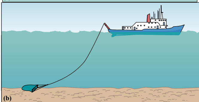
FIGURE 3-10. (a) Rock dredges are used to obtain rock samples, including nodules, from the seafloor with little or no sediment cover. (b) The dredge is lowered on a cable and towed across the seafloor. Sediment passes into and through the net, while nodules and loose rocks are retained. The metal collar breaks off rocks from a rocky seafloor.
