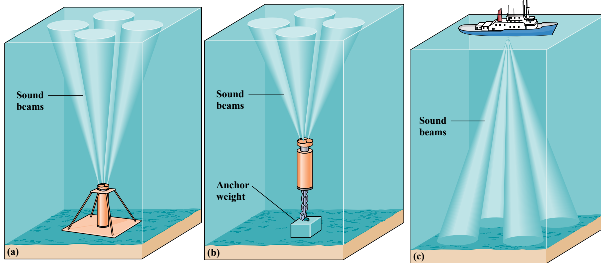
FIGURE 3-18. Doppler acoustic current meters can be (a) mounted on the seabed, (b) moored in mid water, or (c) mounted in a ship's hull facing downward. The sound beams sent out by the meter are reflected off particles in the water, and the frequency of the sound in the returning echo changes according to the direction and speed of the particles that move with the current.
