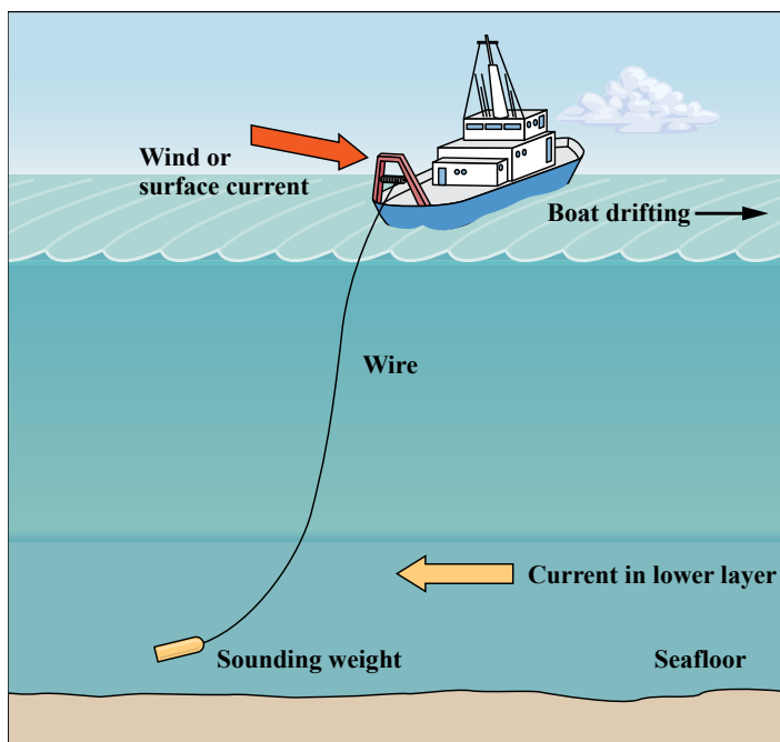
FIGURE 3-2. Winds and currents can deform the vertical path of a sounding weight or instrument package on the end of a wire as it falls to the seafloor. Currents in the surface layer or winds that blow the vessel across the ocean surface can move the vessel away from the vertical path of the weight. Therefore, a length of wire longer than the water's depth must be payed out for the instruments to reach the seafloor. Currents in lower layers can further complicate the path of the wire, particularly in very deep water where several kilometers of wire must be payed out for the instrument package to reach the seafloor.
