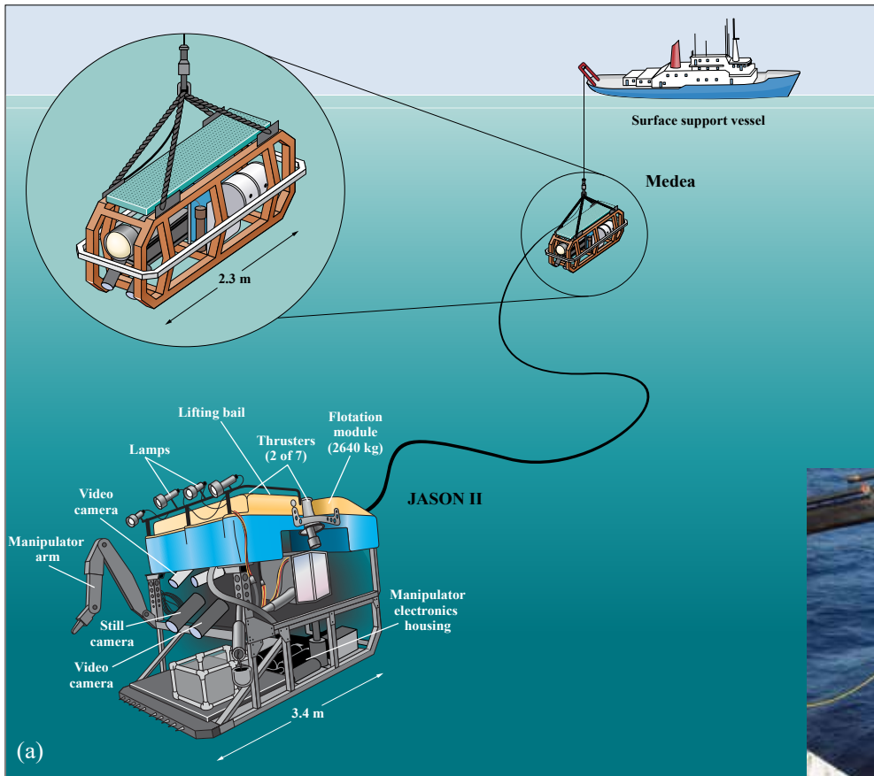
FIGURE 3-24. (a) The Jason II / Medea ROV system. The many motors, instruments, sampling arms, lights, and cameras that are mounted on Jason II and on Medea are operated remotely from a surface vessel. Jason II is connected to Medea by a 35-m-long neutrally buoyant cable and is thus isolated from any ship motions that are transmitted down the cable to Medea . (b) A typical ROV ( Hercules ) can do all the sampling tasks that can be performed by humans in a submersible but at a much lower cost and from smaller vessels.
