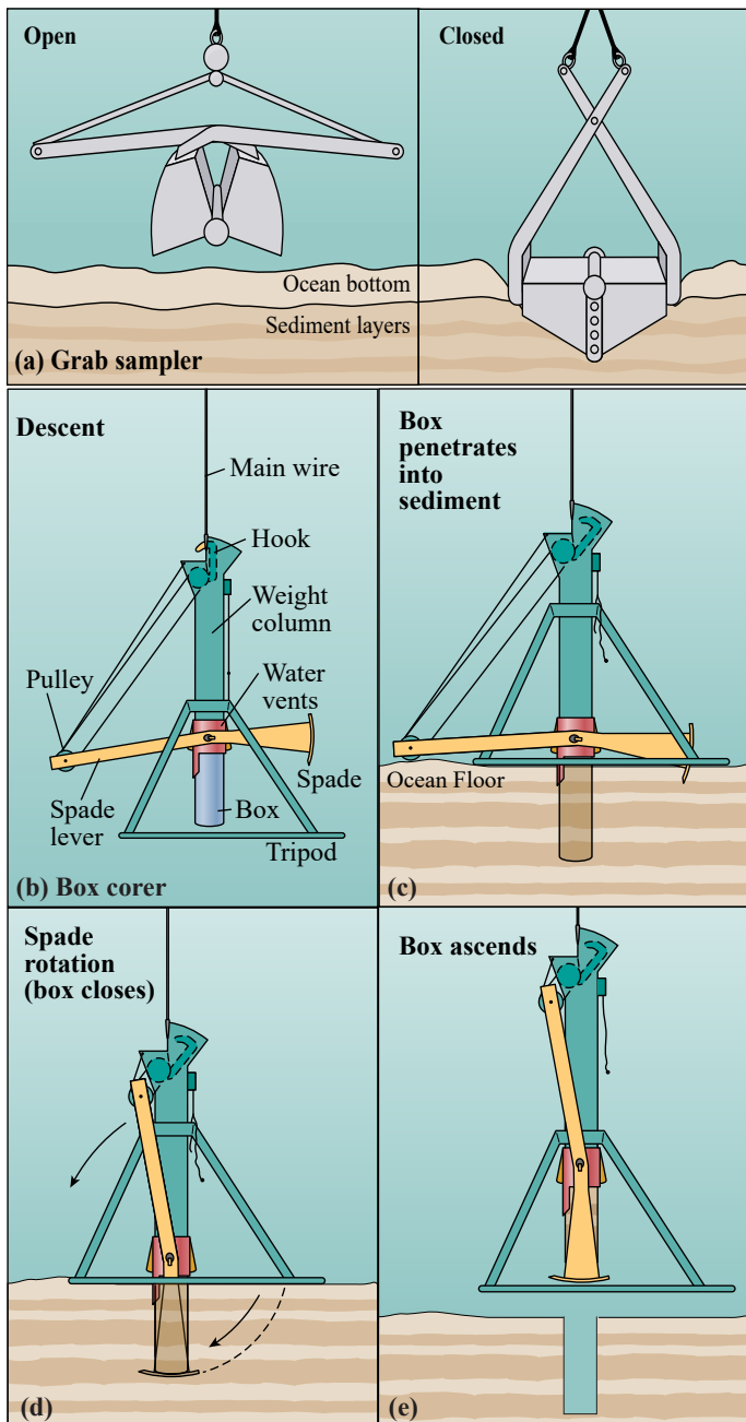
FIGURE 3-7. Methods of sampling near-surface seafloor sediments. (a) Grab samplers are used to obtain large samples of surface sediments. (b) Box corers are used to collect large-volume undisturbed samples of the upper few centimeters of sediment. The box corer is forced into the sediments by its weight and is then closed off by a spade arm that cuts through the sediment and under the box.
