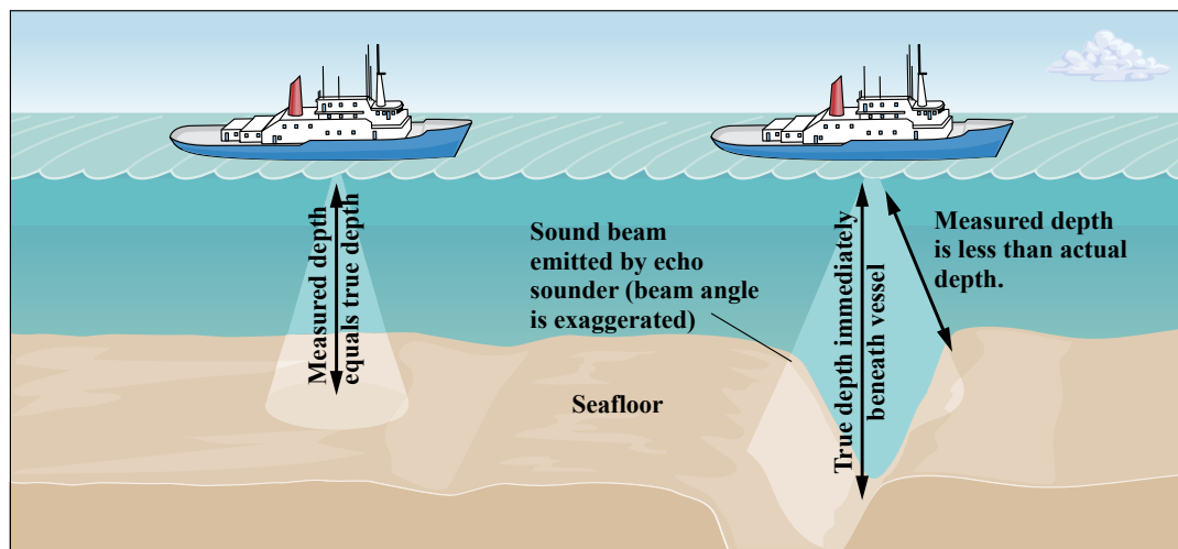
FIGURE 3-3. Echo sounders measure the depth of water beneath a vessel by measuring how much time a sound pulse takes to travel from the vessel to the seafloor and back. Because sound travels in seawater at about 1500 \text{ m}\cdot\text{s}^{-1} , a sound pulse takes 2 s to return to the research vessel when the water depth is 1500 m. The sound pulses spread out over a narrow angle as they travel downward from the vessel. Thus, in deep water, they are reflected off a large area of seafloor.
