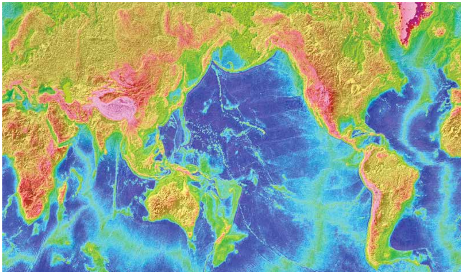
Figure 3-4. Mercator projection map of the seafloor and land surface elevation. Seafloor elevation data were obtained from ship generated precision depth recorder data and satellite measurements of sea surface height data. (Data were obtained from many sources.) The highest resolution sea surface height data used in this map was from satellites, permitting only features greater than about 20–25 km across to be shown in this map. Click for a larger version of the map.
