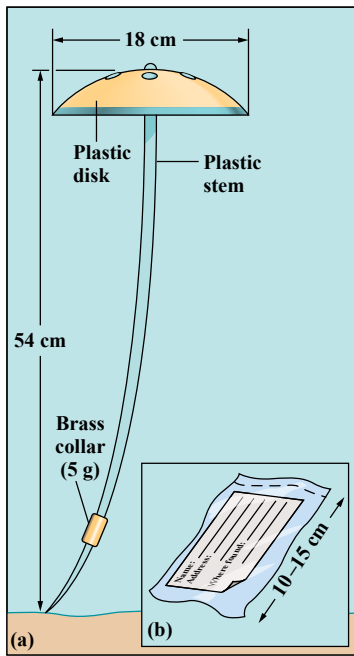
FIGURE 3-15. Surface and seabed drifters can be used to study ocean currents. (a) A seabed drifter is weighted such that its bottom tip drags along the seafloor as the plastic disk section “catches” the current and moves with it, while (b) a surface drift card is usually a simple postage-paid return postcard sealed in plastic that floats flat on the water surface and moves with surface currents.
