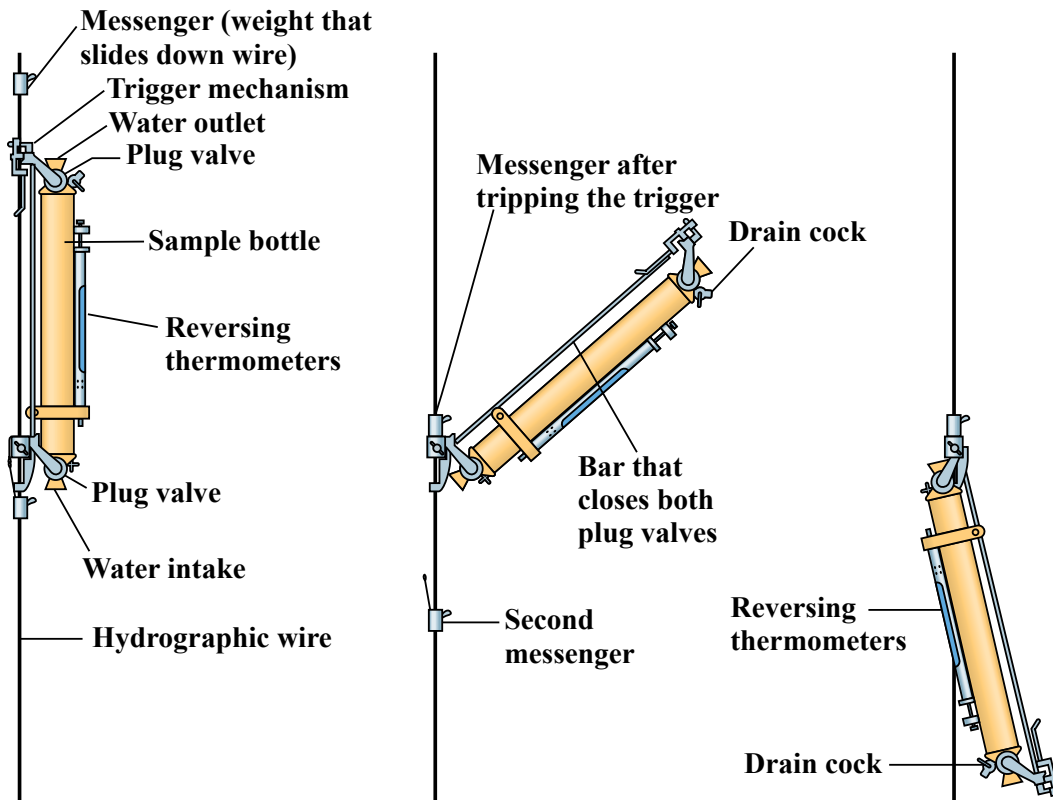
FIGURE 3-11. Nansen water-sampling bottle. When the messenger hits the trigger mechanism, the top of the bottle is released from the wire, the bottle falls into an inverted position, and a mechanical linkage closes valves at each end of the bottle. The trigger mechanism also releases a second messenger, which slides down the wire to the next sampling bottle.
