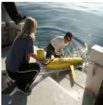
FIGURE 3-26. A Slocum Glider about to be deployed from a research vessel. Basic gliders can be small and easily deployed, while larger gliders can support longer missions and more complex instrumentation
