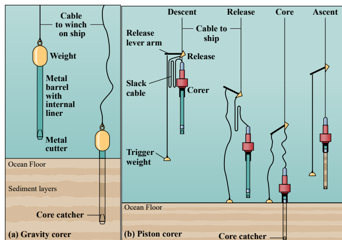
FIGURE 3-8. Sediment corers are used to obtain long, mostly undisturbed, vertical samples of soft seafloor sediments. Most corers have a core catcher that consists of a ring of flexible metal leaves around the inside of the core tip. The leaves are easily pushed aside as the corer enters the sediments, but they are bent backward to close off the tube as the corer is pulled out. (a) Gravity corers are driven into the sediment by their weight and can obtain cores up to about 4 m long. (b) Piston corers are usually suspended from a release arm, which is held in the closed position by a trigger weight that hangs from the end of the trigger arm to below the corer itself. When the trigger weight hits the bottom, the trigger arm is released, allowing the weighted corer to fall freely into the sediments. When the tip of the core barrel reaches the seafloor, a loop of cable between the trigger assembly and a piston inside the core barrel becomes taut holding the piston in position. The movement of the piston causes a small reduction of the water pressure in the barrel above the sediment, helping the sediment core slide into the barrel. The piston mechanism increases core length to longer than 50 m depending on sediment type and minimizes vertical distortion of the sediment layers.
