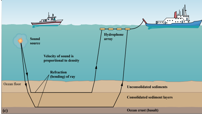
FIGURE 3-9. Two seismic profiling techniques are used to map subsurface sediment layers and structures. (a) Seismic reflection sends sound pulses, which penetrate the seafloor and are reflected off sedimentary layers. (b) A typical reflection seismic profile shows rugged seafloor topography overlaid by sediment layers. (c) Seismic refraction sends sound pulses, which are refracted (bent) at interfaces between layers of sediment and then travel back out to be received by a second ship. At one time, the sound source was provided by dynamite sticks thrown overboard to explode just under the water surface. However, the sound source typically used now is an air gun that periodically fires a burst of compressed air into the water at a depth of about 15 to 35 m. The sound waves are generated by the collapse of the air bubbles produced by each burst. (d) A 3-dimensional seismic refraction image of an ancient reef structure buried beneath the sediments off Nova Scotia, Canada. The light colored 2-dimensional sections across the center of the image and along the right side show how much more information the 3-dimensional image can convey.
