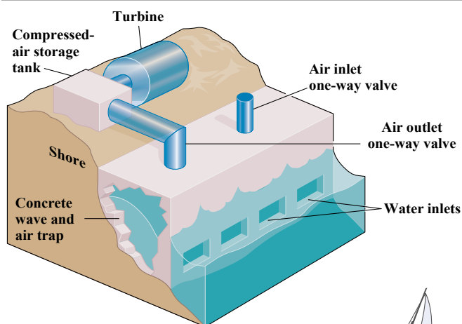
(b) Oscillating water column wave energy converter
