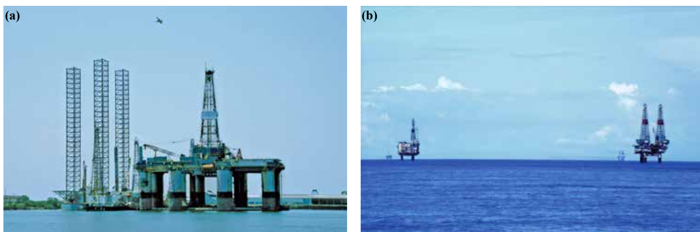
FIGURE 2-13 Structures of the offshore oil and gas industry. (a) These offshore exploration drilling rigs are under maintenance in Galveston, Texas. On the left is a typical jack-up drilling rig; on the right is a typical floating rig that rides on pontoons below the depth of most wave action. (b) Production oil rigs permanently anchored to the seafloor of Cook Inlet, Alaska.
