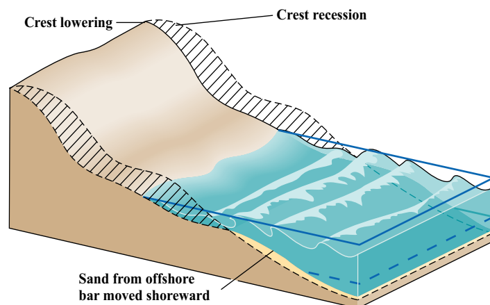
(c) Beach returns to summer profile when wave energy decreases
