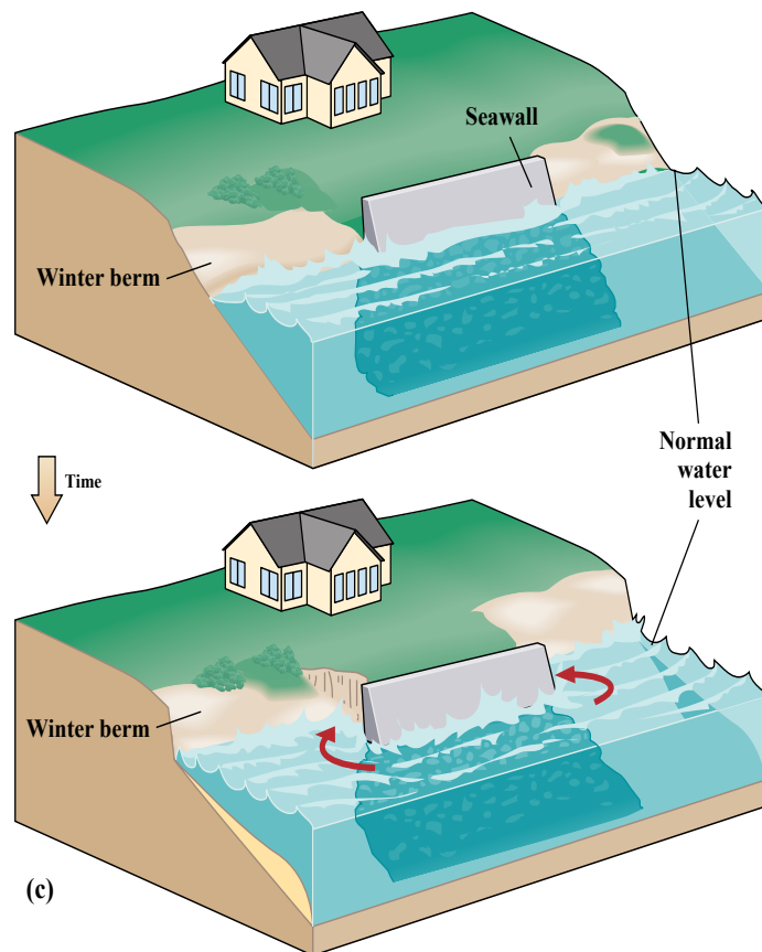
FIGURE 11-23. Seawalls are designed to protect beachfront property from erosion. (a) The Galveston seawall was constructed after the destructive hurricane of 1900. Since the wall was completed in 1962, the beach has eroded along much of its length, leaving the shoreline more exposed to attack by the highest waves of future hurricanes. (b) The barrier island has continued to retreat since the Galveston seawall was constructed. The beach just beyond the end of the wall has now retreated substantially farther shoreward than the wall's location as a result of the natural process of barrier island retreat and the consequent reduction in the amount of sand in the littoral drift system that occurred once the beach had been eroded away in front of the wall. (c) Seawalls are undermined from the sides and eventually destroyed as sea level rises.
