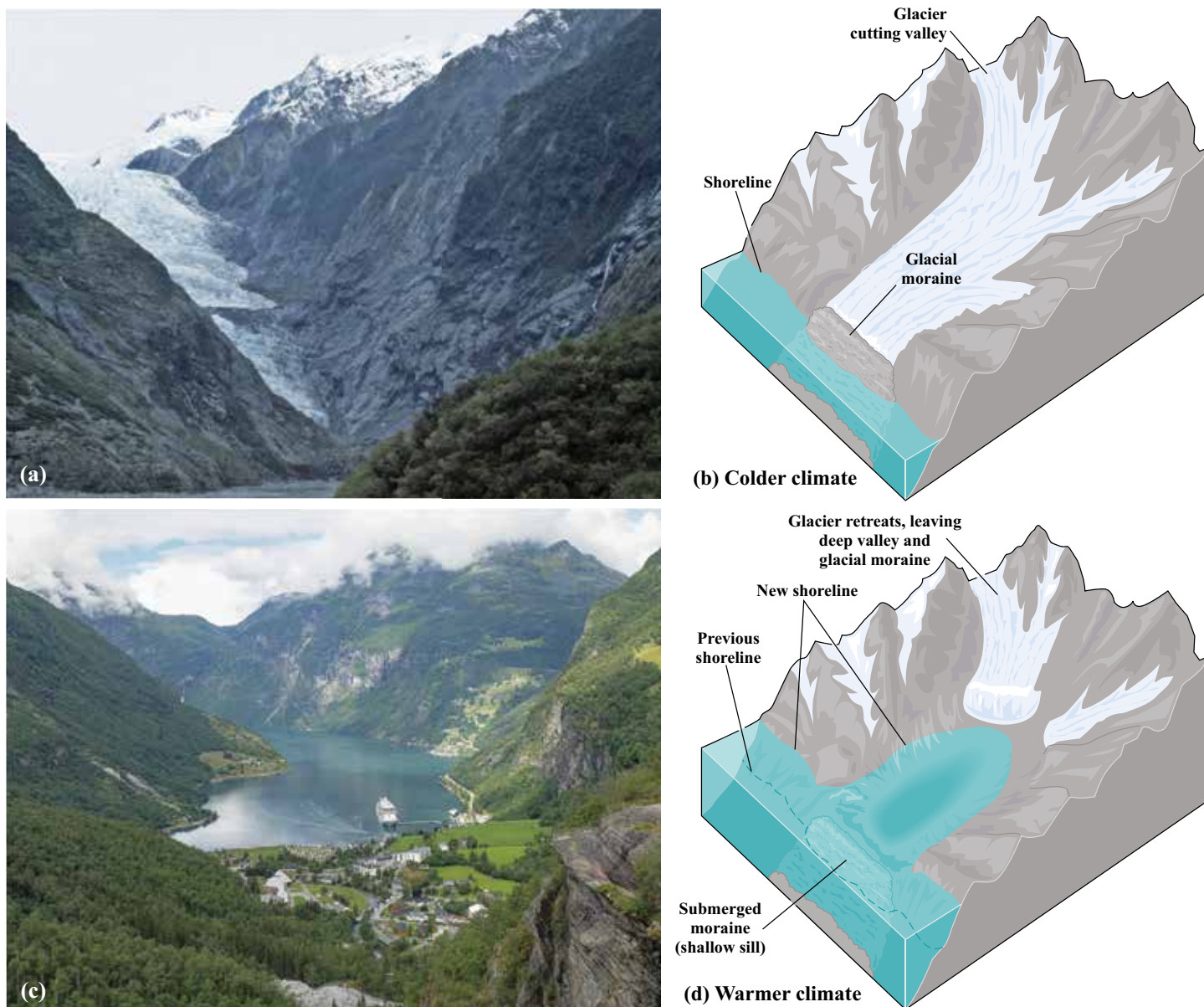
FIGURE 11-6. Glaciers and fjord formation. (a) The Franz Josef Glacier on the South Island of New Zealand has retreated substantially in recent decades. Note the very steep-sided valley that the glacier has left behind as it has receded. (b) When sea level was lower and glaciers more extensive, the glaciers cut deep, steep-sided valleys down to the ancient sea level. Rock fragments carried by the glaciers were deposited to form one or more glacial moraines at the foot of each glacier. (c) Geirangerfjord, Norway where rising sea level has filled a glacial valley that now allows ocean cruise ships to navigate to the head of the fjord, which is 60 km inland. (d) As the Earth's climate warmed and sea level rose, the glaciers retreated, and their steep-sided valleys were filled by seawater to form fjords. The glacial moraines left behind by the glaciers formed shallow submerged sills at the mouths of many fjords.
