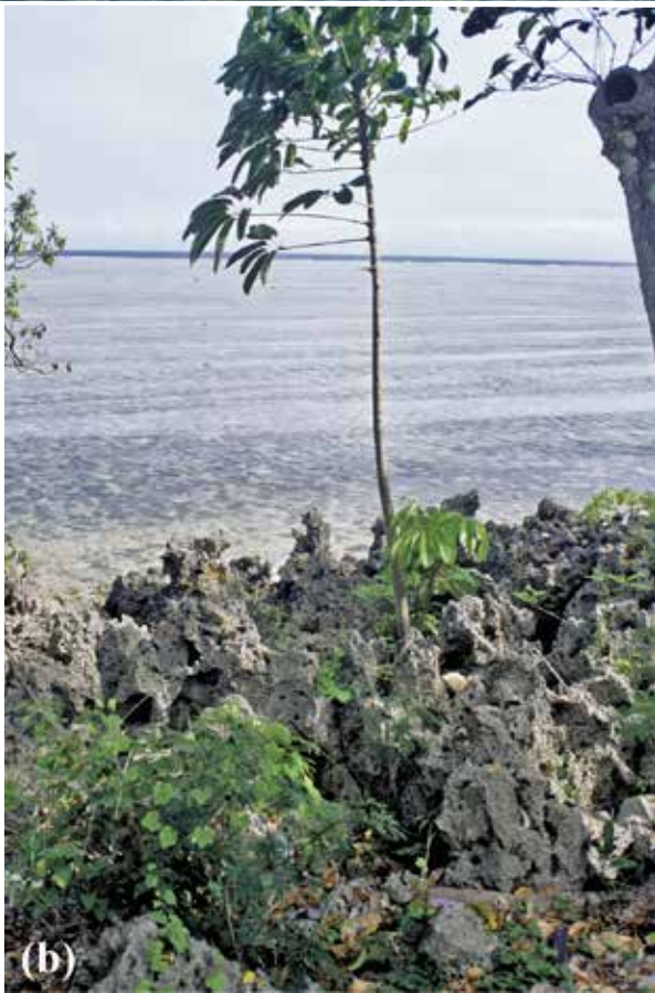
FIGURE 11-8. An uplifted and eroded coral reef forms a jagged shore often called “ironshore.” (a) Coastlines of coral islands, like this island in Palau, often have interspersed sandy beaches and eroding ironshore. (b) The jagged rocks of this ironshore segment in Fiji are razor-sharp.
