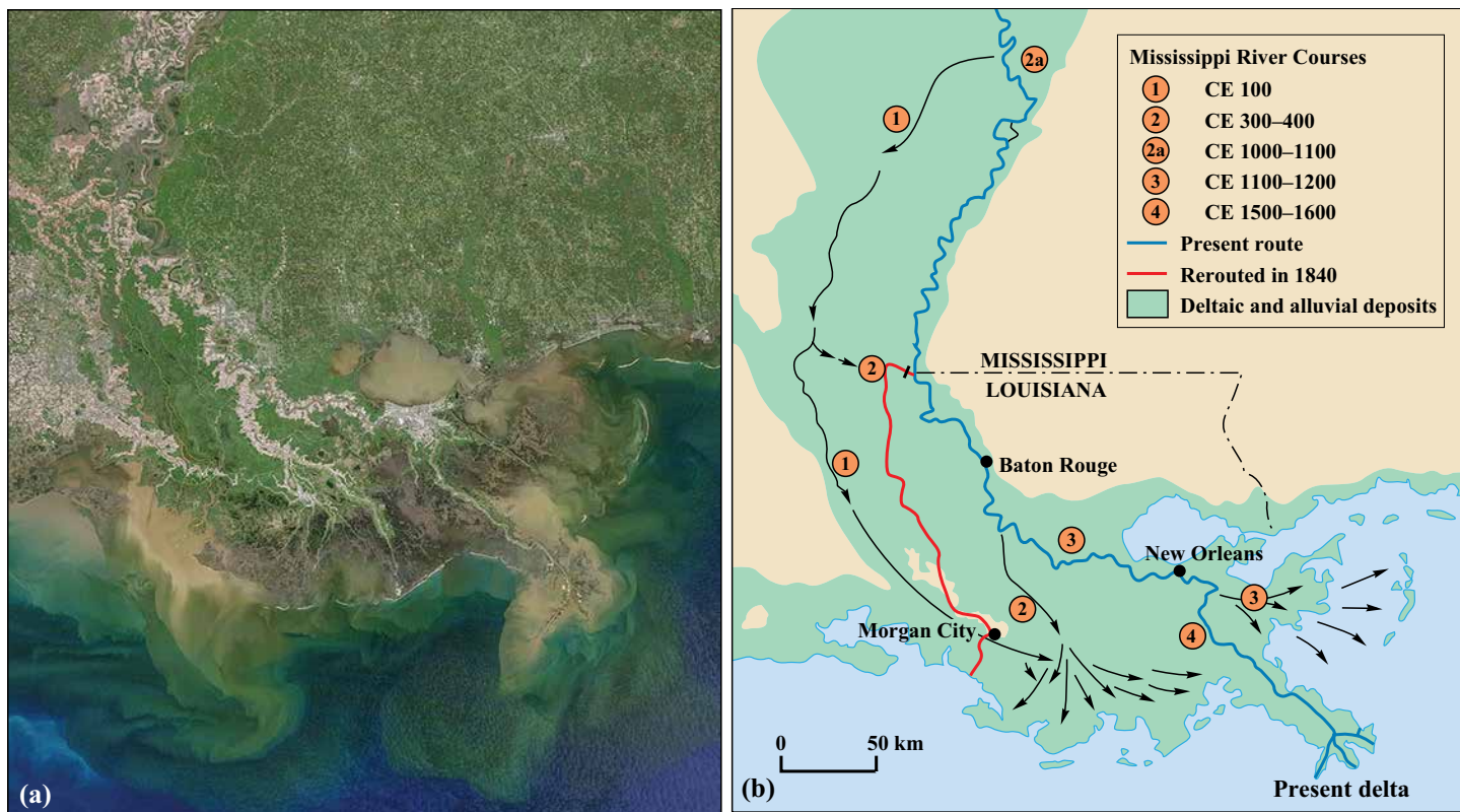
FIGURE 11-7. The Mississippi River delta. (a) This satellite image shows the extensive delta with its many distributary channels. (b) The Mississippi River periodically changes its course through the coastal plain and delta, distributing its sediments across the entire area. Flood-control levees now prevent this natural process.
