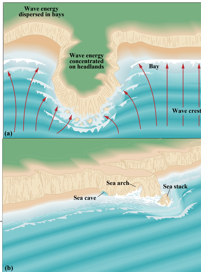
FIGURE 11-12. (a) Wave energy is concentrated on headlands by wave refraction. Because the seafloor topography is rough and varies as slumps occur from different parts of the headland, wave energy is distributed unevenly. In addition, rocks of the headland differ in composition and susceptibility to erosion. As a result, wave action causes the headlands to be eroded unevenly. (b) The uneven erosion of the headland can cause sea caves and sea arches to be formed. (c) This headland on the island of Molokai in Hawaii has been eroded by the intense wave action to form sea caves and sea stacks. (d) There are many sea stacks on the Pacific coast of North America, including these on the Big Sur coast south of Monterey, California.
