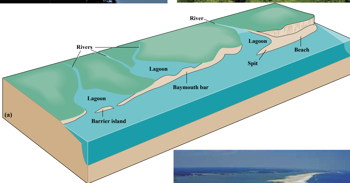
FIGURE 11-21. (a) Spits, baymouth bars, barrier islands, and lagoons are all formed on coastlines where erosion supplies large amounts of sand to the longshore drift. (b) Homer Spit, Alaska. (c) A baymouth bar at the mouth of Tillamook Bay, Oregon. (d) A barrier island, Assateague Island, just south of Ocean City, Maryland looking north.
