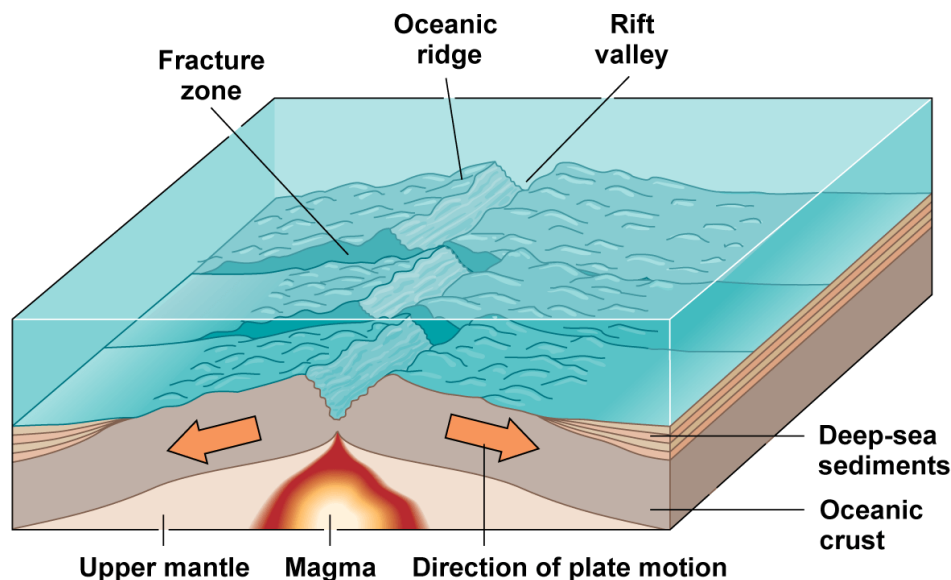
Figure 4-20. Oceanic ridge divergent plate boundaries are characterized by a ridge with a central rift valley and by fracture zones. On slowly spreading ridges, such as the Mid-Atlantic Ridge, the rift valley may be 30 km wide and up to 3 km deep, and the ridge is rugged with steep slopes. On rapidly spreading ridges, such as the East Pacific Rise, the rift valley is typically 2 to 10 km wide and only 100 km or so deep, and the ridge is broad with low-angle slopes and relatively smooth topography.
