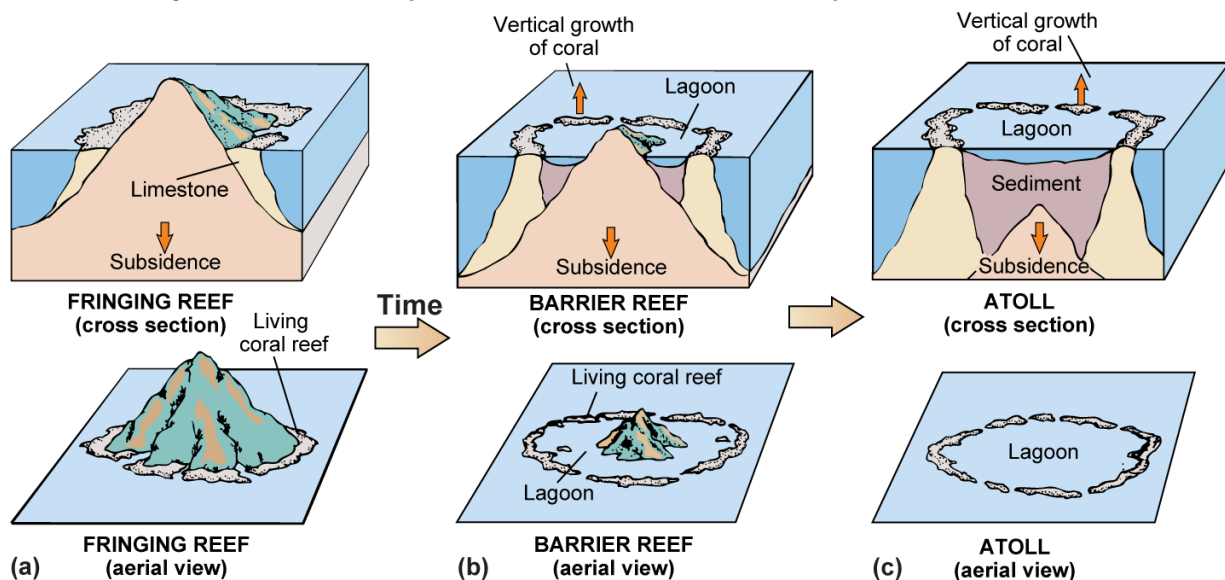
Figure 4-29. Coral reefs form in shallow water in the tropics and subtropics. Reefs are well developed around volcanic islands created at hot spots because there is little runoff of freshwater and sediment, both of which inhibit healthy growth of coral reefs. Coral reefs evolve as volcanic islands are formed and then sink isostatically as they move off the hot spot and cool. (a) Fringing reefs are formed around the perimeter of rising or static volcanic islands. (b) When the island sinks, a barrier reef is formed as the fringing reef grows upward. (c) Eventually, the island sinks completely beneath the surface, leaving an atoll where the barrier reef continues to grow upward.
