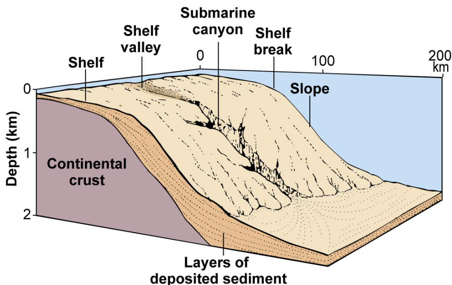
Figure 4-33. The continental shelf is often cut across by shelf valleys, some of which connect to steep-sided submarine canyons that cut across the continental slope.
