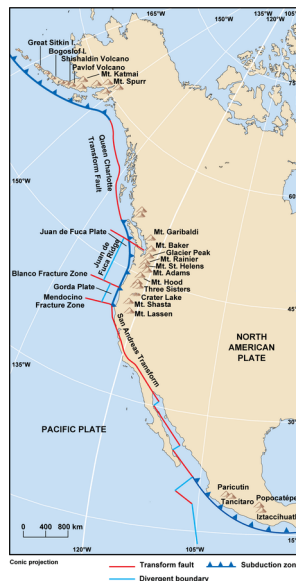
Figure 4-14. Stretches of the west coasts of Mexico, California, Oregon, Washington, Canada, and Alaska are characterized by trenches and continental subduction zone volcanoes. The active volcanoes associated with the subduction of the Juan de Fuca and Gorda Plates under the North American Plate do not extend farther south than Mount Lassen in northern California. To the south, the San Andreas Fault, which can be traced from Cape Mendocino through southern California and into northern Mexico, is a transform fault and not a subduction zone. Continuing southward, active volcanoes are again found in central Mexico, where the transform faults of California end and the subduction zone between the Cocos Plate and the North American Plate begins.
