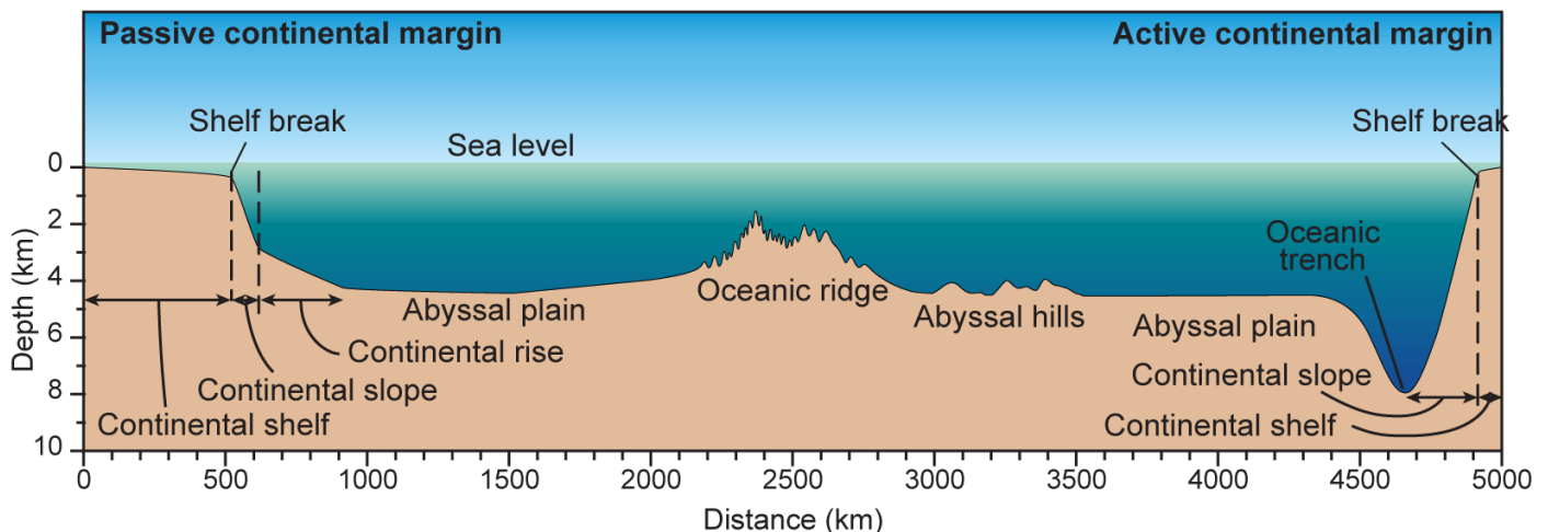
Figure 4-5. General features of the seafloor topography between the continents and the deep ocean floor.
