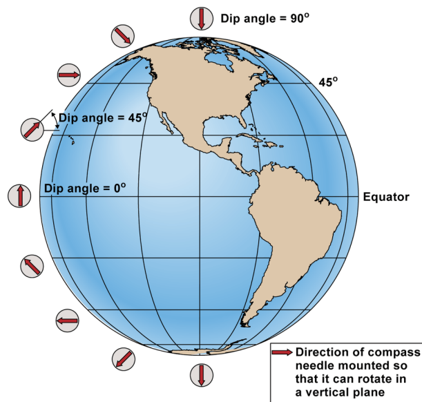
Figure 4-26. The principles of paleomagnetic dip angle. The dip angle is the angle between the rock's direction of magnetization and the Earth's surface (if the rock has not been tilted since being formed). Because the dip angle changes with latitude, the original dip angle of a rock's magnetization reveals the latitude at which it was formed.
