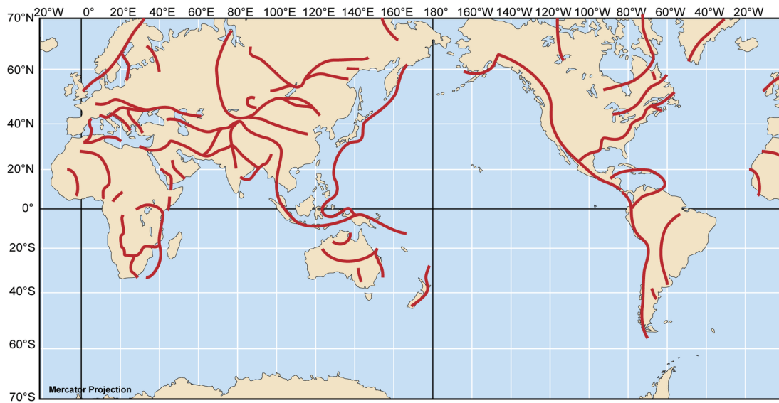
Figure 4-10. Sutures and active subduction zones. Sutures are the remnants of subduction zones where plates once converged. The oldest sutures that have been identified are in the interior of continents and are more than 570 million years old.
