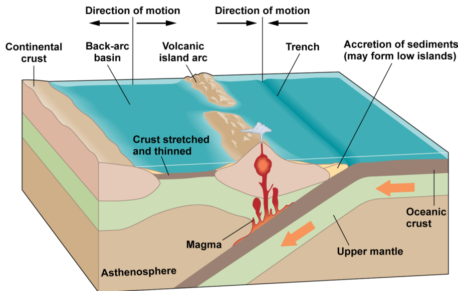
Figure 4-16. At magmatic arc subduction zones, as the plate with the higher-density oceanic crust is subducted, a chain of volcanic islands (magmatic or island arc) is formed along the edge of the nonsubducting plate. Sometimes low sedimentary islands also form between the island arc and the trench. At some magmatic arcs, such as shown here, the oceanic plate subducts fast enough that the adjacent plate (shown with a continental crust edge in this example) does not move toward the plate boundary as fast as the subduction occurs. In this situation, a trench and island arc form outside a back-arc basin, which is created by stretching and thinning of the non-subducting plate edge (the continent edge in this example). The directions of plate motion shown are relative to each other. In some cases, the trench may migrate seaward, while the non-subducting plate migrates more slowly in the same direction so that a back-arc basin is still formed.
