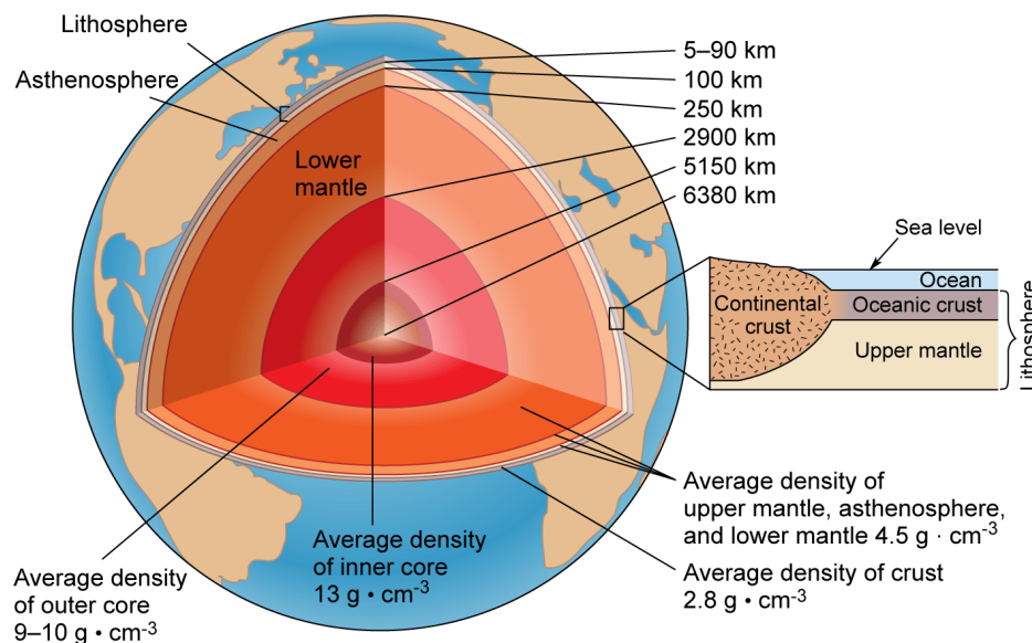
Figure 4-2. A cross section of the Earth showing its layers. Note that the thickness of the lithosphere has been greatly exaggerated in this diagram. If it were drawn to the correct scale, the lithosphere would appear as just a thin line at the Earth's surface.
