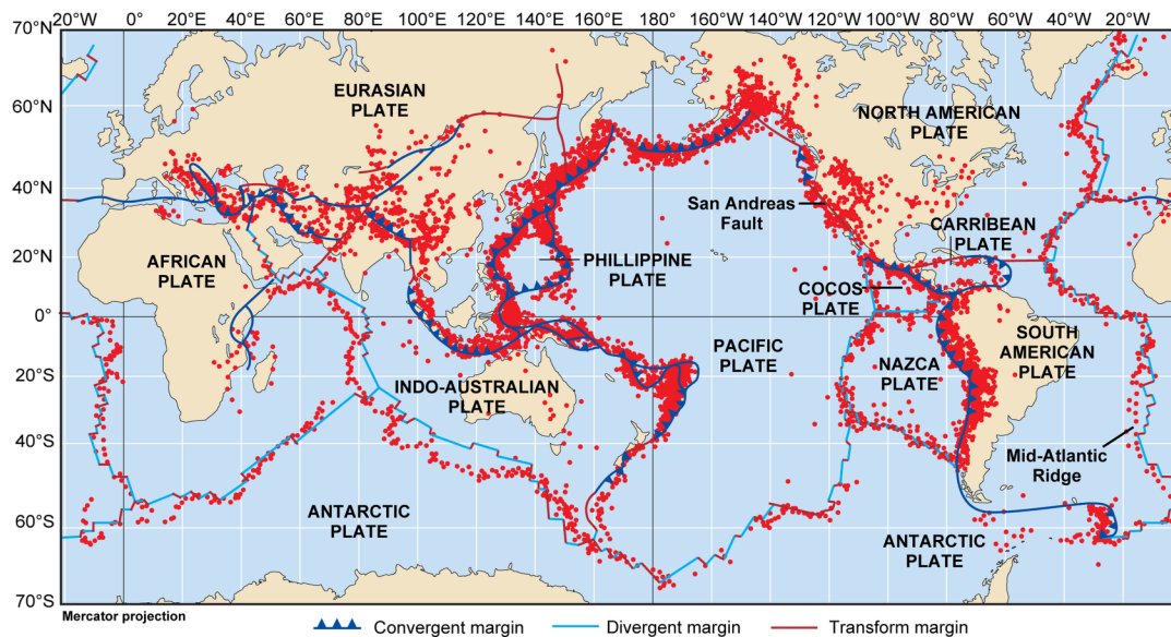
Figure 4-8. Locations of the world's earthquakes. Compare this figure with Figure 4-7. Earthquakes are concentrated along plate boundaries and appear to be more frequent at the plate boundaries where plates are converging.
