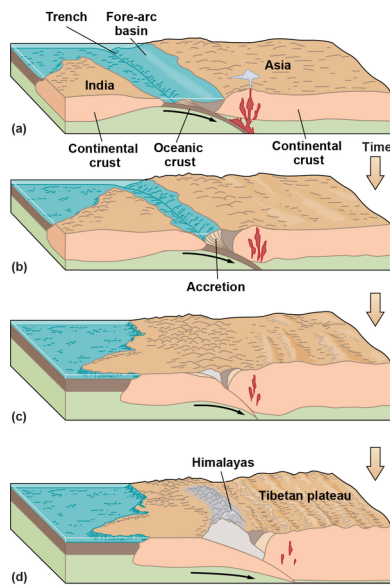
Figure 4-18. The continental collision boundary between India and Asia. About 50 million years ago, the northern margin of the Indian continental crust began a collision with the southern margin of the Asian continental crust. India is being thrust under the Asian continent as the collision continues. The Himalayas and the high Tibetan Plateau were both created by the collision. The tops of the Himalaya Mountains are formed from sedimentary rocks scraped off the oceanic crust of the ocean floor destroyed as the continents first came together.
