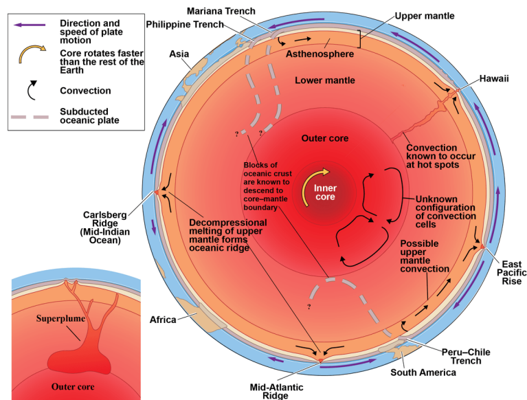
Figure 4-6. A generalized depiction of convection processes thought to occur in the Earth's mantle. The view here is from below the Southern Hemisphere. Not quite half of the Earth has been removed by slicing across the Earth at an angle to the equator. This slice removes much of the Southern Hemisphere, including Antarctica, Australia, much of the southern Atlantic and Indian Oceans, and most of the Pacific Ocean as far north as Hawaii and Indonesia. Look at a globe to see this better. It is known that the convection processes beneath some hot spots extend to the core-mantle boundary, and some subducted blocks of lithosphere may sink to this boundary, but the details of mantle convection circulation are not yet known. Convection cells must exist in the liquid outer core, but almost nothing is known about this circulation. The solid inner core rotates a little faster than the rest of the Earth, making an additional revolution about every 400 years. Scientists believe the faster rotation of the inner core may explain the periodic reversal of the Earth's magnetic field and plate tectonic processes that cause the continents to periodically gather together and then spread apart. However, much research is needed before these processes can be understood. Inset: We know little about superplumes but there are two superplumes at present; in the south Pacific Ocean south of Hawaii (in the part of Earth that is cut off in main figure); and under the African continent (further north than the tip of Africa visible in the main figure). These superplumes are thought to be a "blob" with plumes rising from it as depicted.
