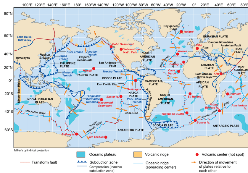
Figure 4-11. The locations of hot spots, subduction zones (trenches), and oceanic ridges. Hot spots occur both at plate boundaries and within plates. Subduction zones occur mostly in the Pacific Ocean, and oceanic ridges are interconnected throughout all of the world's oceans.
