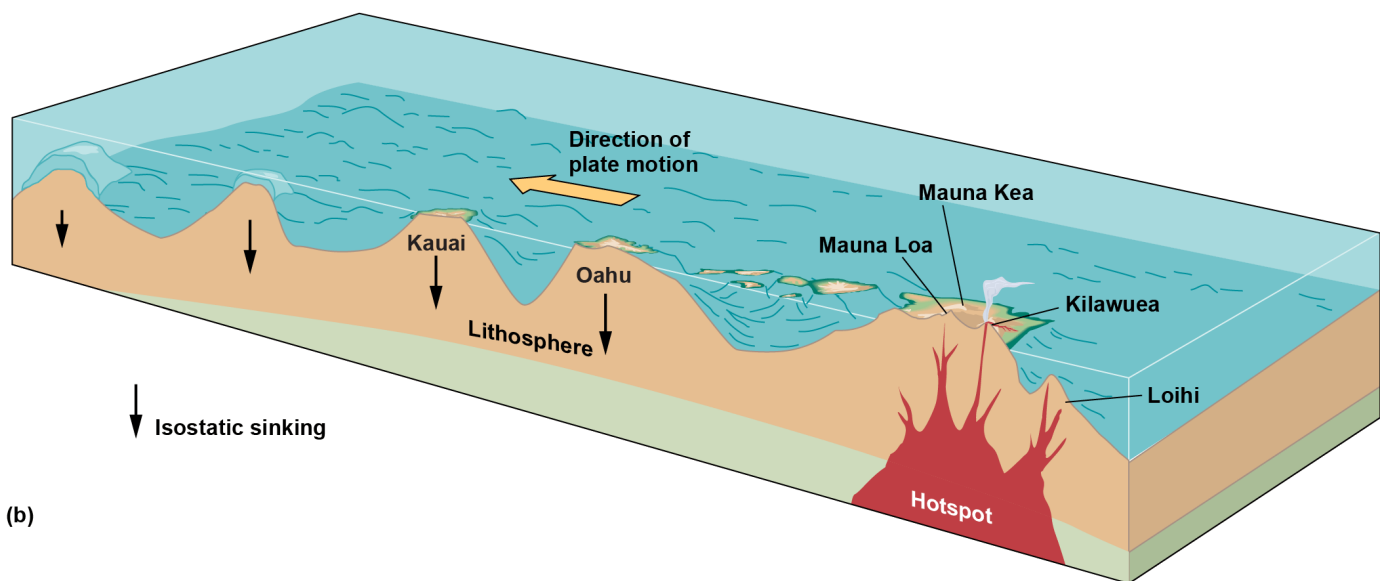
Figure 4-25. (a) The Hawaiian Island-Emperor Seamount chain. (b) The islands and seamounts are formed at the hot spot. As the plate moves relative to the hot spot, new islands are formed, and the older islands move off the hot spot, cool, sink isostatically, and are eroded.
