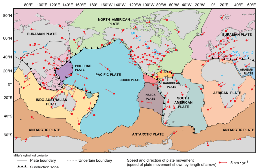
Figure 4-7. The major lithospheric plates and their current directions of motion relative to each other. Continental North America lies on the North American Plate, which extends to the center of the Atlantic Ocean. At the Pacific coast boundary of this plate, the North American and Pacific Plates are sliding past each other. The directions of motion show that the Atlantic Ocean is becoming wider, while the Pacific Ocean is becoming smaller.
