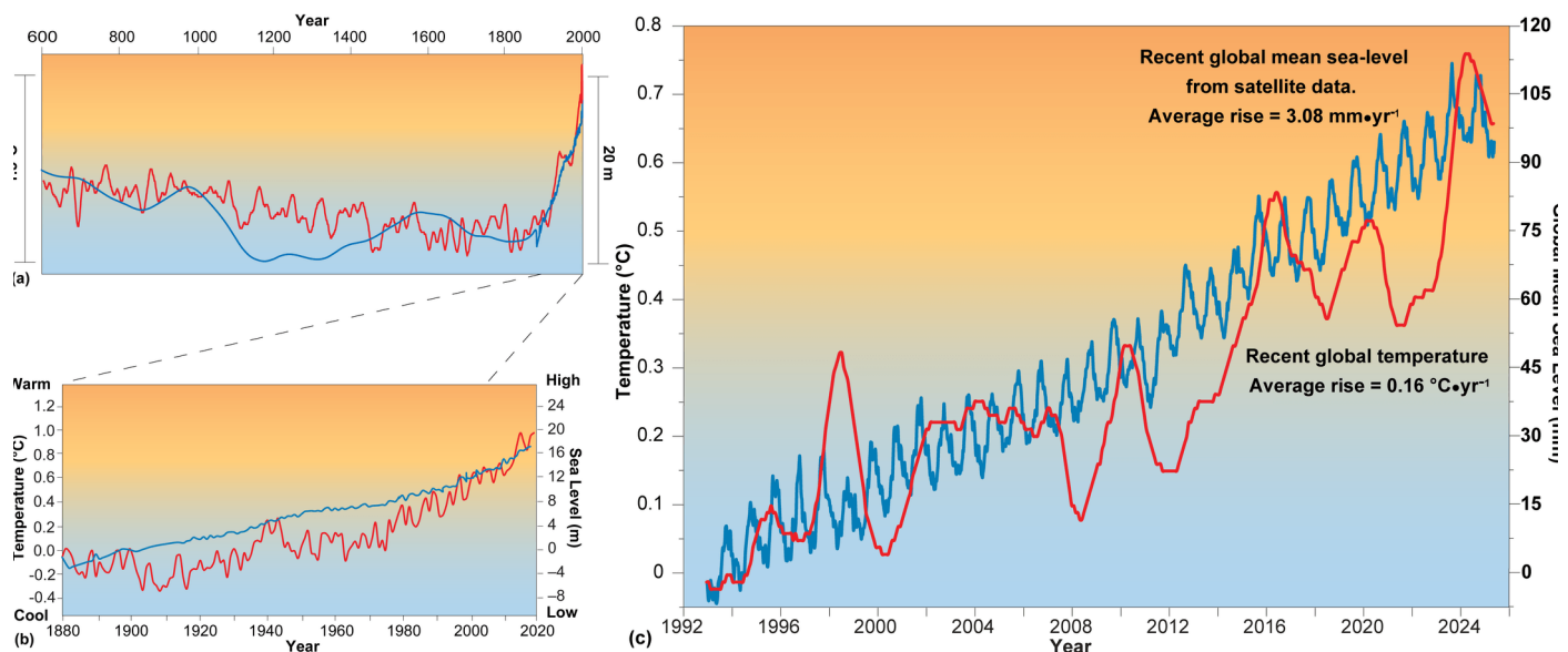
Figure 4-34. Global average surface air temperature and sea level variations within the past 1400 years. (a) Since 600 CE, global average surface air temperature has varied by about 1.5°C, but is currently rising at about 1°C per century. Sea level has varied by about 20 m and appears to follow the trend of temperature changes. (b) Since about 1920, air temperature has started to rise more quickly, as has sea level. However, there is much short-term variability, and the apparent upward trend may not be sustained. (c) Since 1993, instrumental records of temperature show large variations in temperature, but a general increasing trend of 0.16°C·yr -1 . During the same period, highly-accurate satellite measurements show that sea level rise may be accelerating and is now estimated to be about 3 mm·yr -1 . It is not known how far temperature and sea level will rise in the future. It is known that the temperature increase and sea level rise are due to a combination of natural change and the enhanced greenhouse effect but it is not clear what the relative contributions of these two factors has been. This raises the question as to whether the rate of sea level rise could accelerate substantially if the current rising temperature trend is sustained.
