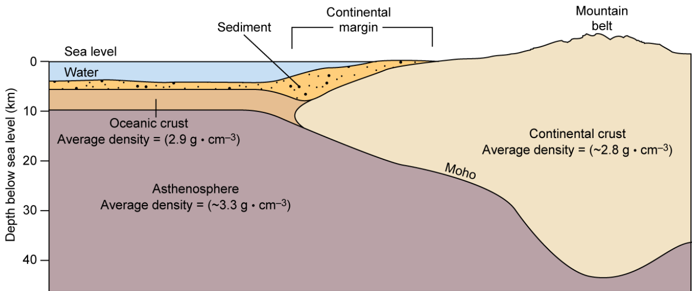
Figure 4-3. Structure of the lithosphere. Continental crust is typically 35 to 40 km thick, whereas oceanic crust is typically only 6 to 7 km thick. Continental crust has a lower density than oceanic crust, but both continental and oceanic crust have a considerably lower density than upper mantle material.
