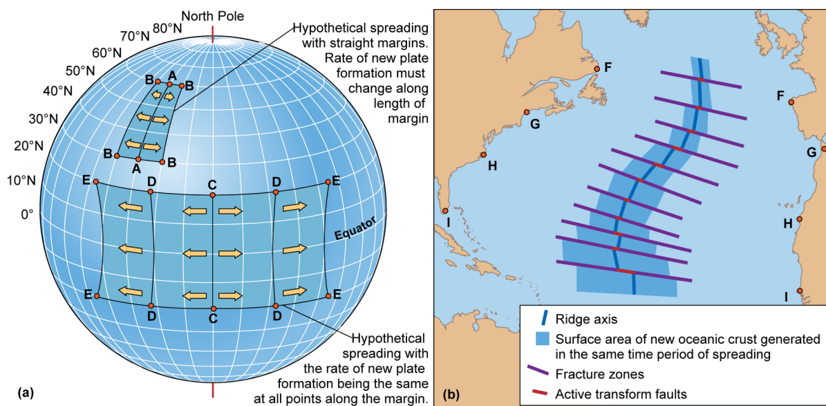
Figure 4-22. (a) Because lithospheric plates have rigid shapes and move on a spherical surface, they must rotate with respect to each other, and the rate of formation or destruction of crust at any plate boundary must vary along the plate boundary's length as shown by the spreading from A to B in this figure. The principle is similar to the movement of your eyelids as you open and close your eyes. The eye is exposed or covered more rapidly at the center than at the two corners. The rate of spreading cannot be equal along the plate boundary because the plates would need to bend and deform. This is shown by the vertical lines through the sequence C–D–E, which represent where the plate divergent boundary would be if spreading were uniform along the plate boundary. (b) Each of the points labeled with the same letter on either side of the Atlantic Ocean were joined at one time. Since the pairs are now separated by different distances, crust must have been formed at different rates along the oceanic ridge. Because the lithosphere is rigid and cannot stretch along its edge, variation in the rate of formation or destruction of crust is accommodated by the formation of transform faults between segments of the plate boundary.
