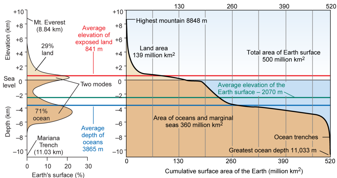
Figure 4-4. Relative heights of parts of the Earth's surface. The average elevation of the continents is 841 m above sea level, and the average depth of the oceans is 3865 m. Almost 30% of the Earth's surface is above sea level. Much of the surface of the continental crust is below sea level.
