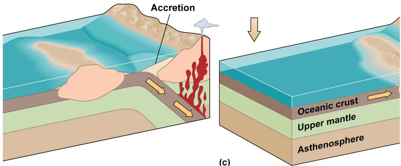
Figure 4-15. Formation of exotic terranes. Oceanic plateaus, inactive oceanic ridges, and volcanoes are scraped off the oceanic crust as it enters a subduction zone. The scraped-off material forms new continental crust that is welded onto the edge of the continent and is called an exotic terrain.
