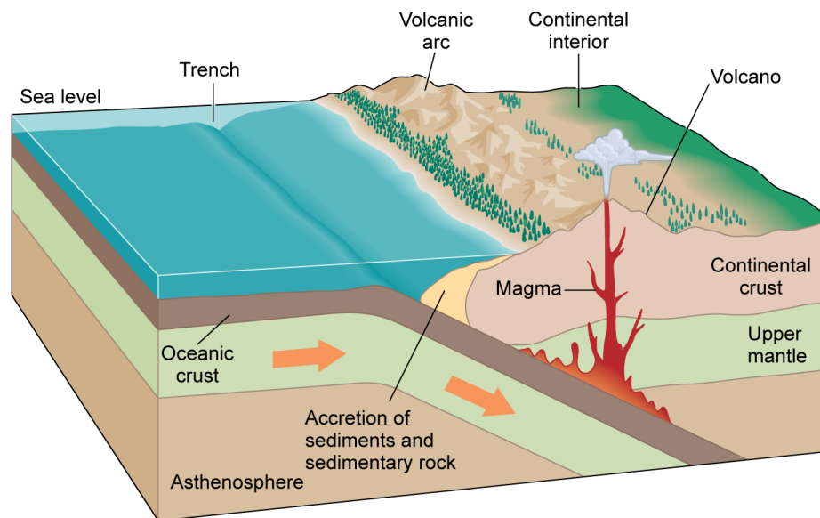
Figure 4-12. Subduction zone at a continental margin. A plate with oceanic crust is subducted beneath a plate with continental crust. This process forms a trench, a chain of volcanoes near the edge of the continent, and a chain of coastal hills or mountains, which are formed by compaction of the continental crust edge and accretion of compacted sediments and sedimentary rock from the subducting plate.
