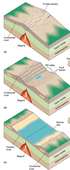
Figure 4-21. The history of new ocean formation at a rift zone. (a) Rising magma beneath a continent pushes the crust upward and creates cracks and fractures. (b) The crust is stretched and thinned. Collapses occur along a series of fault blocks, leading to the formation of a rift valley. Lakes may be formed in the rift valley. (c) The rift widens, allowing ocean water to enter and creating a narrow sea, such as the Red Sea. The rift continues to widen, and an oceanic ridge is formed down its center, eventually creating a new ocean.
