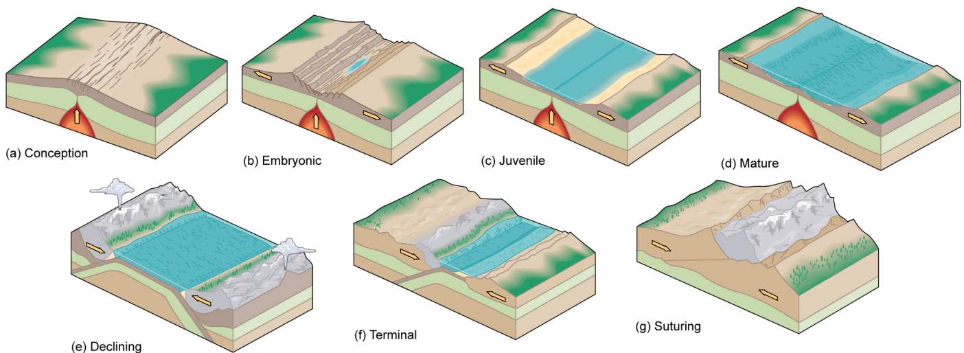
Figure 4-27. The history of an ocean from its creation at an oceanic ridge to its disappearance at a continental collision.
