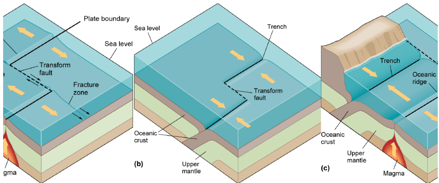
Figure 4-23. Adjacent plates move past each other at a transform fault. (a) Most transform faults connect two segments of an oceanic ridge. The plates slide past each other in the region between the two ridge crests. This is the transform fault. Beyond this region, the two ridge segments are locked together and form a fracture zone. A transform fault can also connect (b) two adjacent segments of a trench or two trenches, or (c) an oceanic ridge and a trench.
