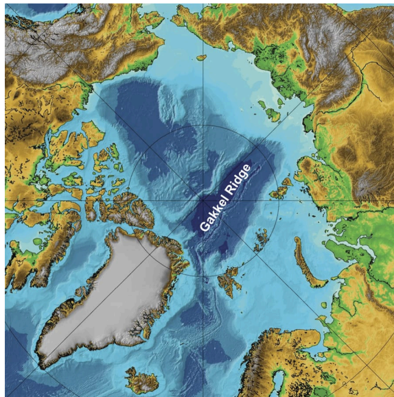
Figure 4-19. Topography of the Arctic Ocean floor. The Mid-Atlantic Ridge extends into the Arctic Ocean. This extension is named the Gakkel Ridge. Shallow sills restrict water circulation between the Arctic Ocean and other oceans. The sill between the Arctic Ocean and the Bering Sea is especially shallow, and the circulation between the Arctic and Pacific Oceans is more restricted than the circulation between the Arctic and Atlantic Oceans.
