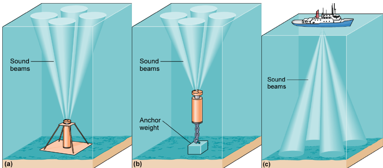
Figure 3-18. Doppler acoustic current meters can be (a) mounted on the seabed, (b) moored in mid water, or (c) mounted in a ship's hull facing downward. The sound beams sent out by the meter are reflected off particles in the water, and the frequency of the sound in the returning echo changes according to the direction and speed of the particles that move with the current.
