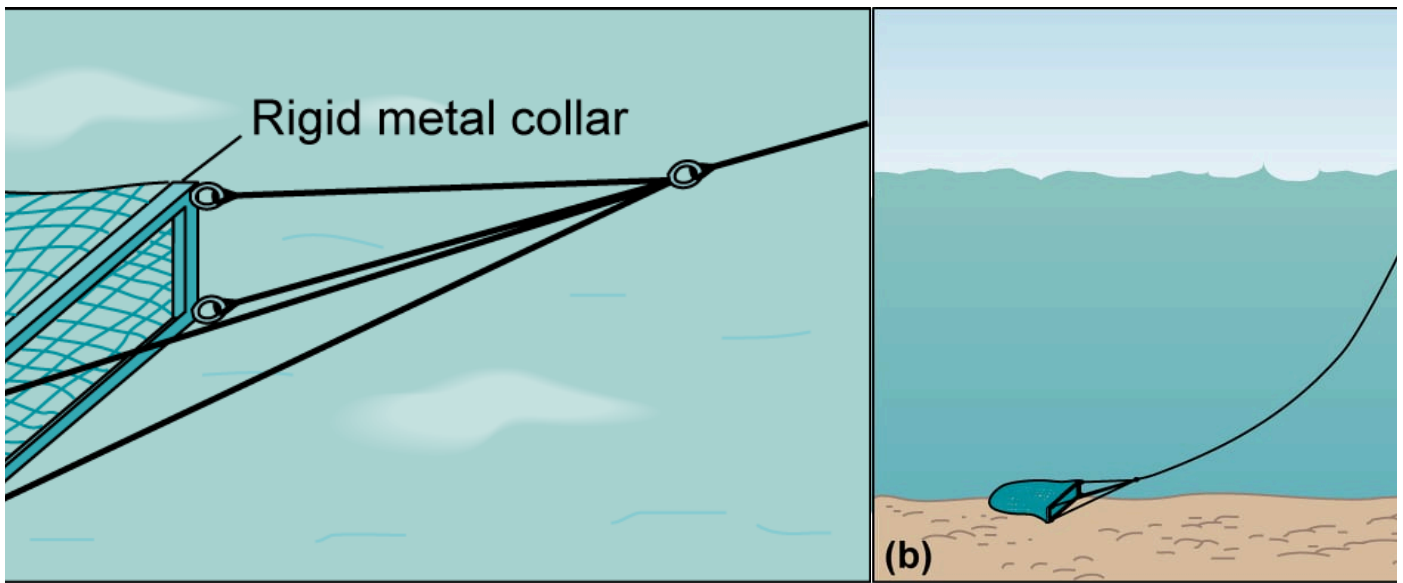
Figure 3-10. (a) Rock dredges are used to obtain rock samples, including nodules, from the seafloor with little or no sediment cover. (b) The dredge is lowered on a cable and towed across the seafloor. Sediment passes into and through the net, while nodules and loose rocks are retained. The metal collar breaks off rocks from a rocky seafloor.
