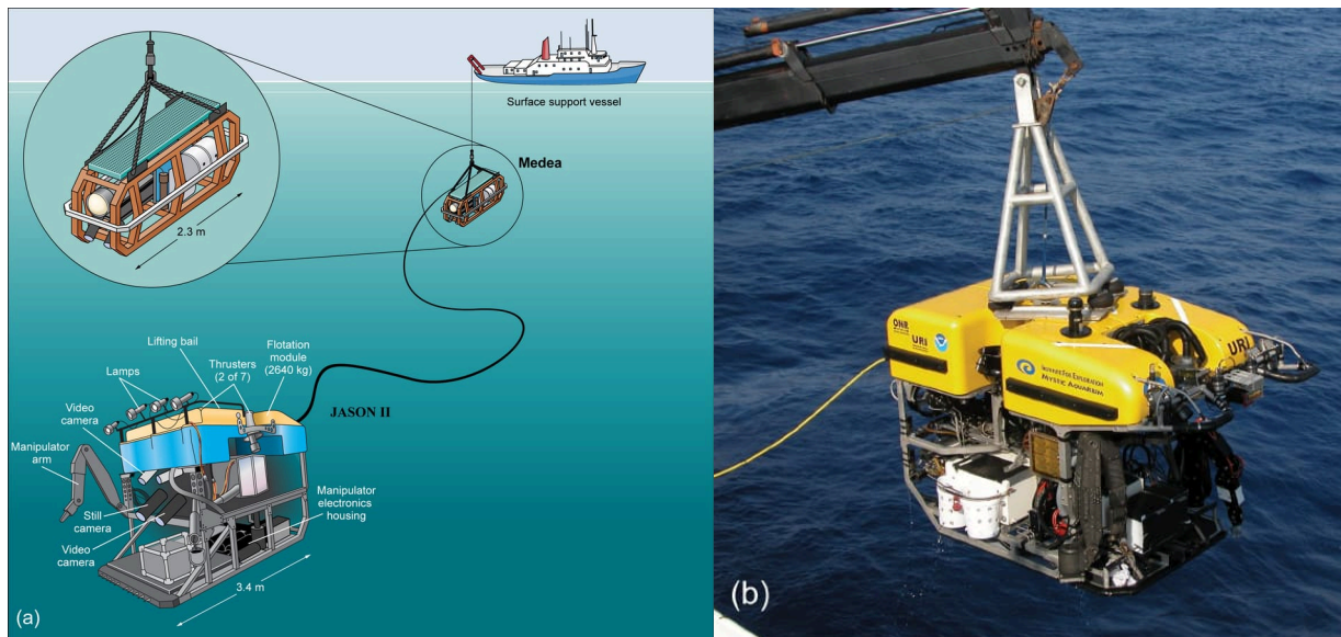
Figure 3-24. (a) The Jason II / Medea ROV system. The many motors, instruments, sampling arms, lights, and cameras that are mounted on Jason II and on Medea are operated remotely from a surface vessel. Jason II is connected to Medea by a 35-m-long neutrally buoyant cable and is thus isolated from any ship motions that are transmitted down the cable to Medea . (b) A typical ROV ( Hercules ) can do all the sampling tasks that can be performed by humans in a submersible but at a much lower cost and from smaller vessels.
