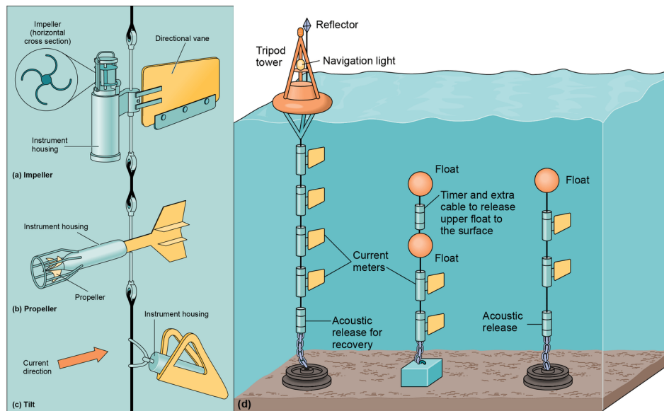
Figure 3-17. Typical designs for current meters measure current speed by recording the (a) rate of rotation of a rotor that behaves much like a waterwheel (this type of rotor is known as a “Savonius rotor” or an “impeller”), (b) rate of rotation of a propeller, and (c) angle to which the meter is pushed by the current. Vanes or fins are used to orient the meter in the current. Current speed and direction are usually recorded on tape in the meter and are read when the meter is retrieved. (d) Current meters are typically deployed in vertical strings, such as the three different configurations shown here, all moored to the seafloor. They are often left in place for weeks or months and then retrieved by activating a timer or an acoustic signal from the recovery ship to release the bottom weights. Often current meters are moored entirely below the surface to discourage theft and to reduce navigation hazards.
