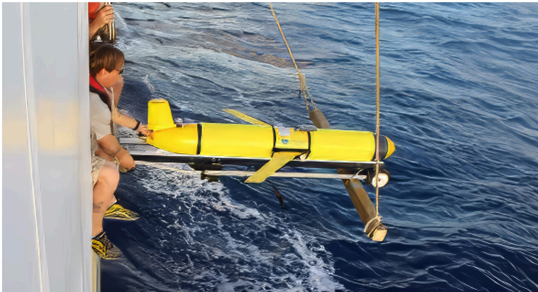
Figure 3-26. A Slocum Glider about to be deployed from a research vessel. Basic gliders can be small and easily deployed, while larger gliders can support longer missions and more complex instrumentation.
