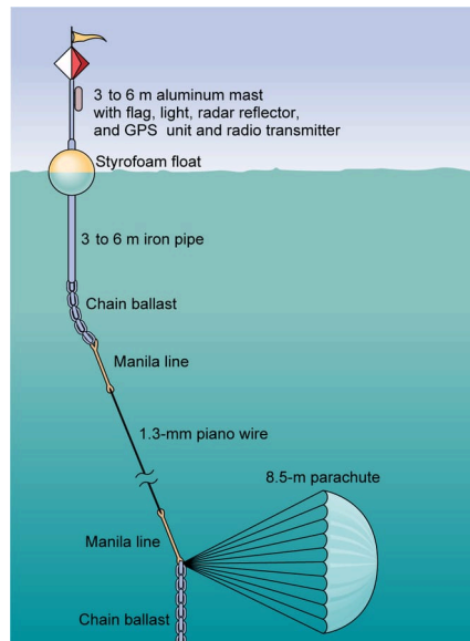
Figure 3-16. A parachute drogue consists of a parachute deployed at a selected depth (usually less than 100 m), where it sails along with the current. The parachute is attached to a surface float that drags the surface float after it. The researchers can follow the changing position of the float using visual observations, radar from a ship, or remotely using a GPS unit and radio transmitter mounted on the float.
