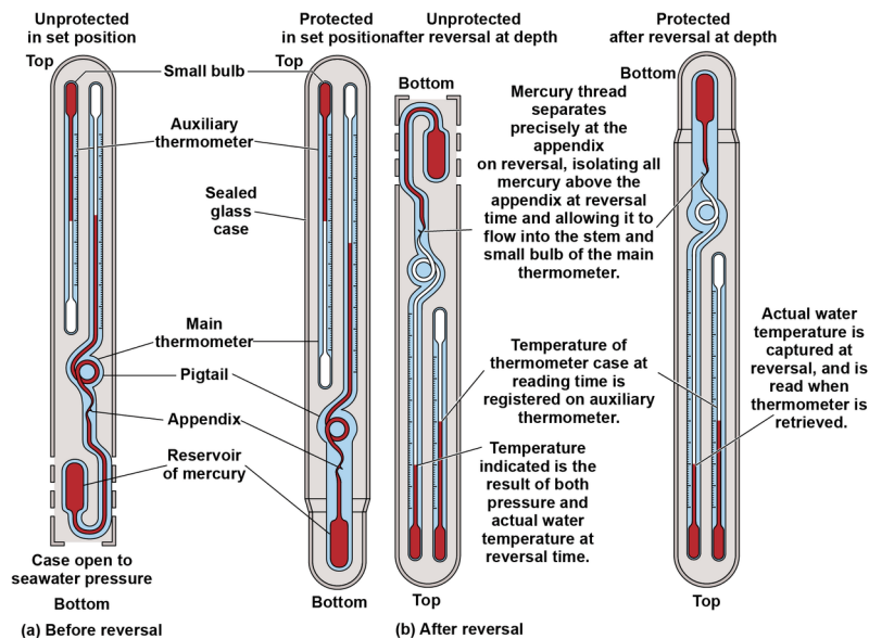
Figure 3-13. (a) Reversing thermometers like these are attached in their set position to a water-sampling bottle in a rack. (b) When the bottle is closed, the rack and thermometers are turned upside down (reversed). The protected thermometer records the true temperature, while the unprotected thermometer records a temperature that is slightly too high because the mercury reservoir is squeezed slightly by the increased pressure at depth. The temperature difference between the thermometers can be used to determine the depth at which the thermometers were reversed. Reversing thermometers are still used to calibrate CTDs, which are instrument packages that measure conductivity, temperature, and depth electronically.
