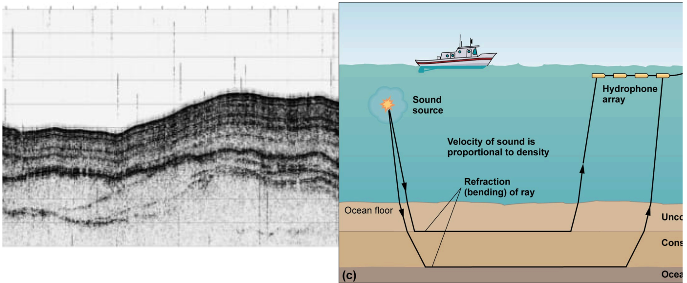
Figure 3-9. Two seismic profiling techniques are used to map subsurface sediment layers and structures. (a) Seismic reflection sends sound pulses, which penetrate the seafloor and are reflected off sedimentary layers. (b) A typical reflection seismic profile shows rugged seafloor topography overlaid by sediment layers. (c) Seismic refraction sends sound pulses, which are refracted (bent) at interfaces between layers of sediment and then travel back out to be received by a second ship. At one time, the sound source was provided by dynamite sticks thrown overboard to explode just under the water surface. However, the sound source typically used now is an air gun that periodically fires a burst of compressed air into the water at a depth of about 15 to 35 m. The sound waves are generated by the collapse of the air bubbles produced by each burst. (d) A 3-dimensional seismic refraction image of an ancient reef structure buried beneath the sediments off Nova Scotia, Canada. The light colored 2-dimensional sections across the center of the image and along the right side show how much more information the 3-dimensional image can convey.
