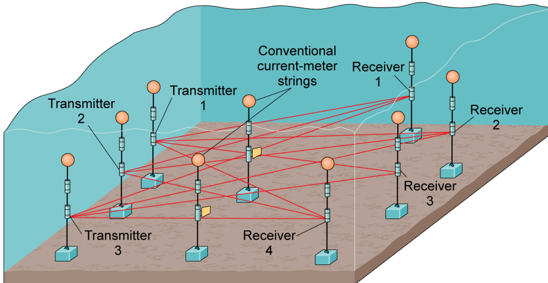
Figure 3-19. In a typical acoustic tomography array, sound pulses are sent from each transmitter and received by each of the receivers.
