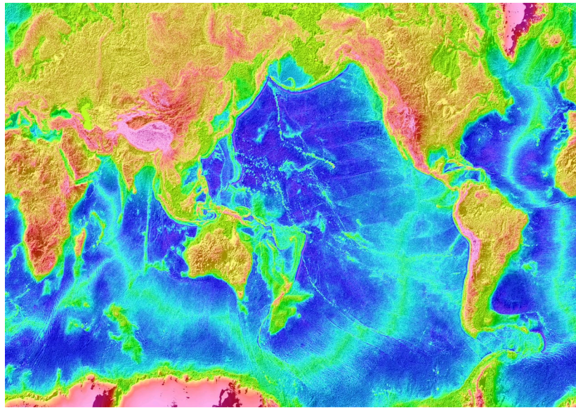
Figure 3-4. Mercator projection map of the seafloor and land surface elevation. Seafloor elevation data were obtained from ship generated precision depth recorder data and satellite measurements of sea surface height data. (Data were obtained from many sources.) The highest resolution sea surface height data used in this map was from satellites, permitting only features greater than about 20–25 km across to be shown in this map. Click for a larger version of the map.
