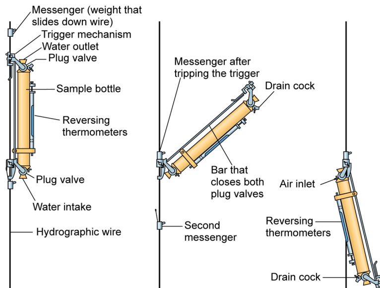
Figure 3-11. Nansen water-sampling bottle. When the messenger hits the trigger mechanism, the top of the bottle is released from the wire, the bottle falls into an inverted position, and a mechanical linkage closes valves at each end of the bottle. The trigger mechanism also releases a second messenger, which slides down the wire to the next sampling bottle.
