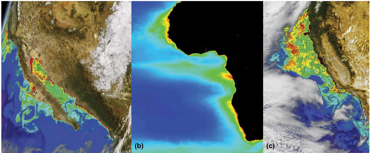
Figure 13-7. These false color-enhanced satellite images show the elevated (red colors) chlorophyll concentrations associated with the interaction of coastal currents and capes. (a) The complex eddies that form at capes and that support enhanced primary productivity are clearly seen in this monthly composite image of the coastal region off Baja California. (b) Upwelling is especially strong and extends farther offshore at each of the several capes on the western African coast. (c) This image shows the intense upwelling that sustains the abundant marine species populations of the California coastal zone. This, and other eastern boundary current coastal upwelling zones, are difficult to capture from satellites since they are often obscured by the marine layer clouds and fog that you can see offshore in the image and that characterize these zones.
