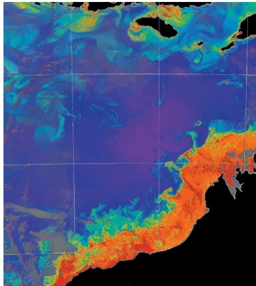
Figure 13-6. Surface water chlorophyll concentrations in the Indian Ocean between Indonesia and northwestern Australia (June 1981). High concentrations are shown in red and are associated with high rates of primary production. The high productivity off northwestern Australia occurs because winds cause offshore Ekman transport and coastal upwelling. Note the complex local variations along the coast. The productivity is much lower near Indonesia, where there is no major coastal upwelling.
