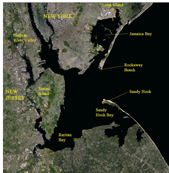
Figure 13-19. This satellite image of the Hudson River basin–New York Harbor–Raritan Bay estuary shows the complex character of this estuary. The Hudson River valley is a glacier-cut valley that was then shaped by a river and so can be considered a coastal-plain estuary. Parts of the river are steep-sided and deep enough that they may even be considered a fjord. Sandy Hook Bay and Jamaica Bay are bar-built. Raritan Bay and New York Harbor could be considered either coastal-plain estuary segments or bar-built, or both.
