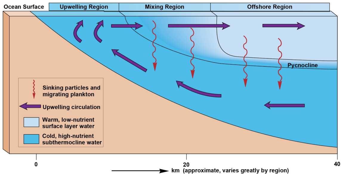
Figure 13-8. In coastal upwelling regions, the distribution of water properties and biota is related to the upwelling circulation. Upwelled water, high in nutrients, supports only low levels of primary production at first, but as it moves offshore as the surface layer, it supports a diatom bloom that depletes the nutrients, after which flagellates become dominant. Zooplankton and fish species are distributed to take advantage of this distribution of food. Many species of plankton use the upwelling circulation by changing their depth to be transported either onshore or offshore. Many fish and invertebrate species also use the circulation by placing their eggs and larvae at the right place and depth so that they are transported to a location where the appropriate food source is available at the different stages of their life cycle.
