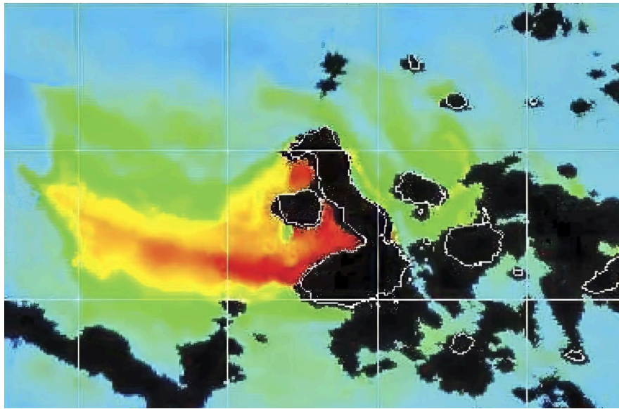
Figure 13-10. Elevated chlorophyll concentrations are found around islands, including the Galápagos Islands, which are depicted in this false color-enhanced satellite image. Primary productivity is enhanced by the vertical mixing that is caused by the interaction of ocean currents with the island topography, which brings nutrients to the surface layer, and by nutrients in freshwater runoff from the islands.
