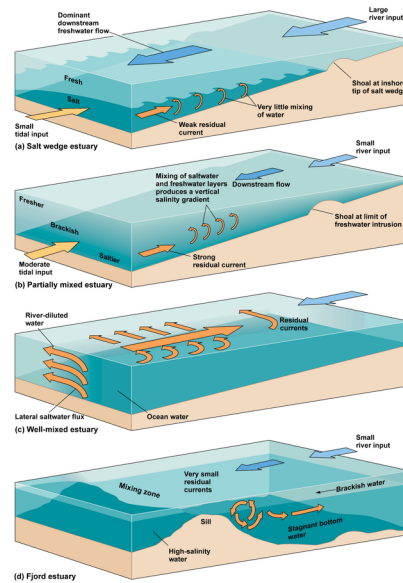
Figure 13-21. Types of estuaries categorized by circulation pattern. (a) Salt wedge estuaries are characterized by a net (after tidal motions are averaged out) landward current in the lower layer and a net seaward current in the upper layer. There is little vertical mixing, but breaking internal waves on the halocline mix some seawater up into the surface layer. (b) Partially mixed estuaries are characterized by relatively strong net landward currents near the seafloor and relatively strong net seaward currents in the lower salinity (fresher) surface layer. (c) Well-mixed estuaries have no vertical salinity variations, but they do have variations in salinity both across and down the length of the estuary. The Coriolis effect causes net estuarine currents to flow landward at all depths on the right side of the estuary in the Northern Hemisphere (viewed from the ocean), and seaward flow at all depths on the left side. These currents are on the reverse sides in the Southern Hemisphere. (d) Estuaries in fjords have little current in the deep water below the depth of any sill. In the upper layers above the sill depth, there is generally a salt wedge or sometimes a partially mixed estuary circulation pattern.
