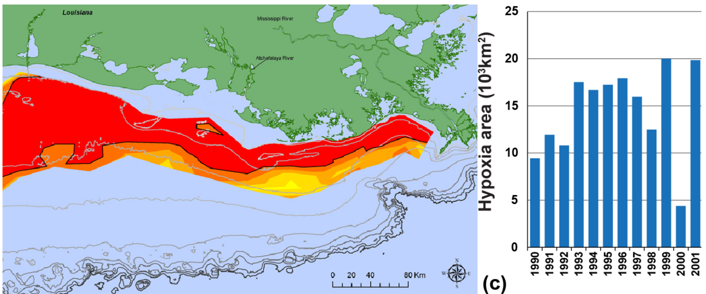
Figure 13-15. Anoxia. (a) During the summer of 1976, eutrophication and unusual climate conditions combined to produce anoxia, or conditions in which oxygen concentrations were too low to support animal life (values of less than 2 in this figure), throughout a large area of the New Jersey continental shelf. This event caused the deaths of massive numbers of clams and other benthic fauna. (b) Hypoxia and anoxia now occur annually each summer in a large area of the Gulf of Mexico continental shelf. This map shows the extent of the hypoxia, commonly referred to as a dead zone, in summer of 2017, the largest area to date. Levels of oxygen above 2.0 are considered essential for marine animals to survive. (c) The Gulf of Mexico dead zone affects an area of the Gulf that varies in extent each year. However, the area is now comparable to or greater than the maximum area of fisheries closures during the Deepwater Horizon oil spill of 2010.
