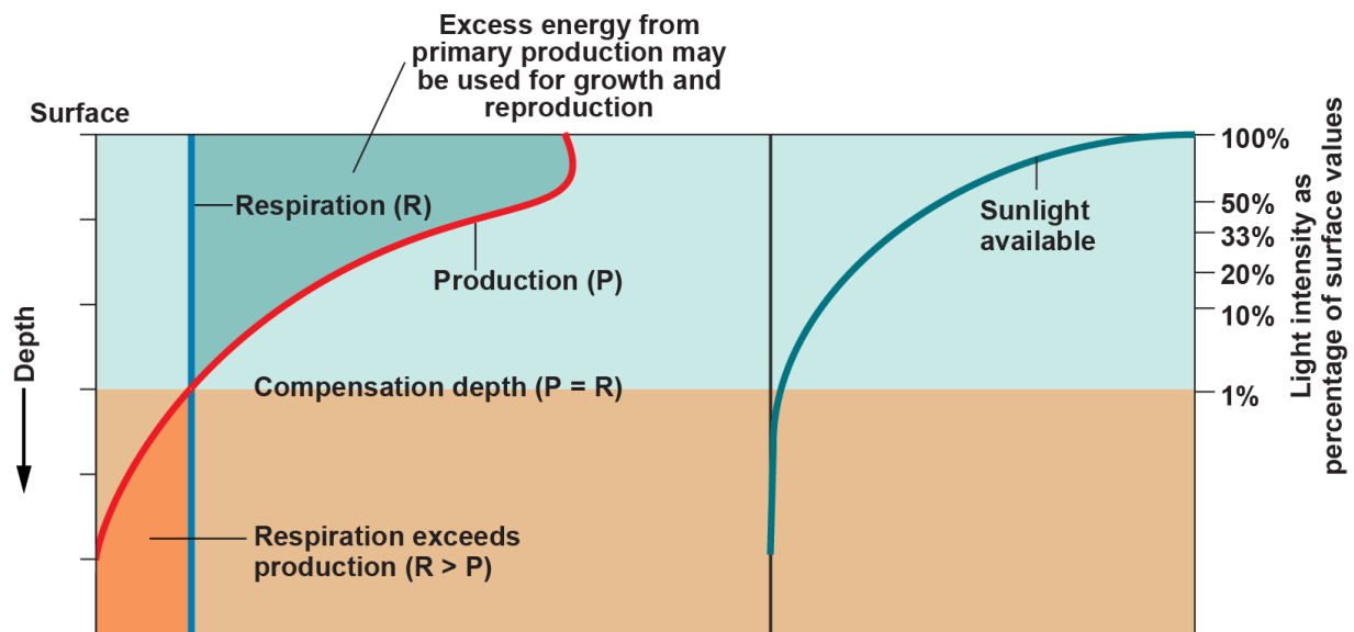
Figure 12-5. Photosynthesis depends on the availability of light energy. Therefore, the rate of primary production by phytoplankton decreases with decreasing light intensity and, thus, with depth. The rate of metabolic energy use and, thus, respiration by phytoplankton remains almost constant regardless of depth. The depth at which the rate of phytoplankton primary production equals the rate of phytoplankton respiration is called the “compensation depth.” Below this depth, phytoplankton use more organic matter for respiration than they can produce by photosynthesis. The water column above the compensation depth is the photic zone, and everything below this depth is in the aphotic zone.
