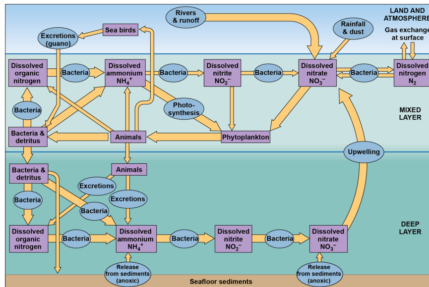
Figure 12-7. Simplified representation of the nitrogen cycle in the oceans. The boxes represent compartments (CC10) or components of the system among which the nitrogen is distributed. The ovals represent processes that transport the nitrogen or convert its chemical form between these compartments. Thicker arrows show more important pathways. Unlike phosphorus, nitrogen is not recycled rapidly in the photic zone, and it tends to be transported below the thermocline. Thus, nitrogen is often the limiting nutrient. Nitrogen can be recycled from shallow seafloor sediments (as depicted for phosphorus in Figure 12-6), but these pathways have been omitted in this figure to reduce its complexity.
