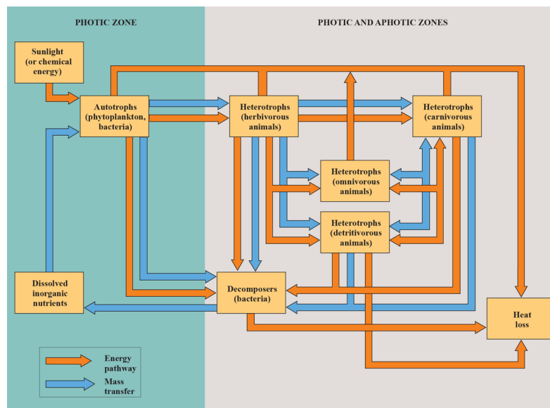
Figure 12-3. Simplified model of the energy and mass (organic matter and nutrient element) cycles in a marine ecosystem. Sunlight (or chemical energy) and dissolved nutrients are essential for autotrophs to perform the phototrophic (or chemosynthetic) primary production of organic matter from carbon dioxide. Energy collected and mass produced by autotrophs is cycled through various heterotrophs, followed by decomposers. The mass is transferred back to solution by decomposers, and the energy is eventually released as heat. Primary production of organic matter takes place only in the photic zone (except for limited areas where chemosynthesis occurs). All other steps in the ecosystem take place partly in the photic zone and partly in the aphotic zone.
