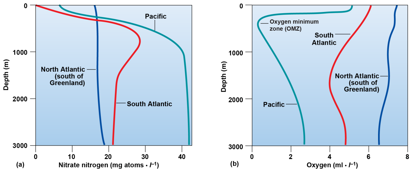
Figure 12-9. The vertical profiles of nitrate nitrogen and dissolved oxygen in the North Atlantic (south of Greenland), South Atlantic, and North Pacific Oceans are very different. In the North Atlantic, where cooled surface water is sinking to form North Atlantic Deep Water (NADW), the concentrations vary little with depth. During its passage southward to the South Atlantic, this water mass loses oxygen and gains dissolved nitrate as respiration by animals and decomposers uses oxygen and releases dissolved nitrate. This process continues as the water mass moves around Antarctica and northward into the deep water of the Pacific Ocean. Thus, the ratio of nitrate concentration to oxygen concentration is an indication of the “age” of the water mass since it left the surface layer. Higher ratios indicate “older” water. The “oldest” water has too little oxygen for animal life to survive in and areas with this low level of oxygen are called oxygen minimum zones (OMZs).
