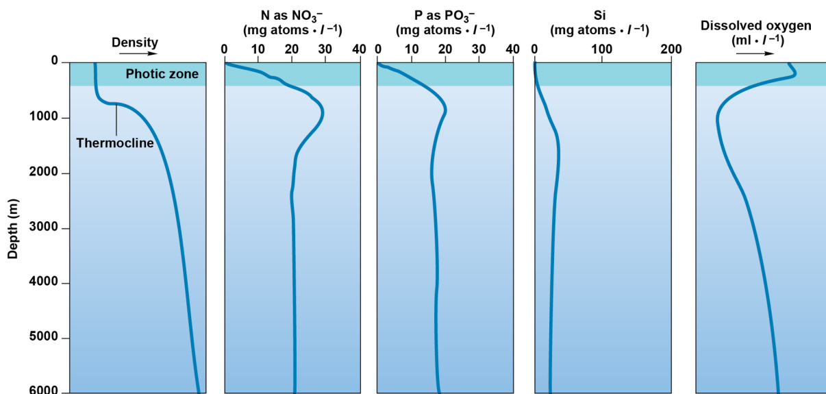
Figure 12-8. General representation of the vertical profiles of water density, nitrate, phosphate, silicate, and dissolved oxygen concentrations in the center of the Atlantic Ocean basin. Dissolved oxygen concentration is high above the thermocline, reaches a minimum just under the thermocline, and then increases to somewhat higher levels in the deep water masses formed by cooling of surface water at high latitudes. Nutrients (nitrate, phosphate, silicate) are generally depleted in the photic zone, increase rapidly in concentration until they reach a maximum at about the same depth as the dissolved oxygen minimum, then remain at relatively constant high levels in the deep water masses.
