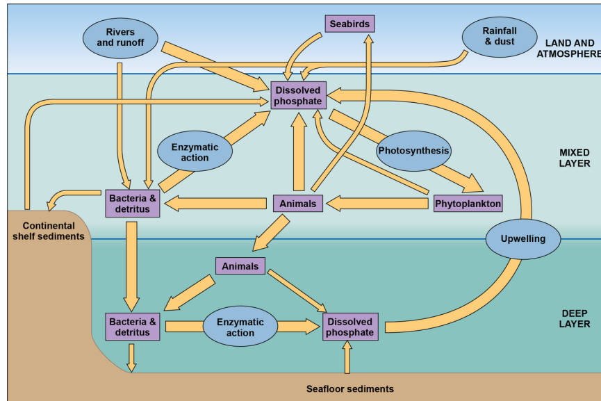
Figure 12-6. Simplified representation of the phosphorus cycle in the oceans. The boxes represent compartments (CC10) or components of the system among which the phosphorus is distributed. The ovals represent processes that transport or convert the phosphorus between these compartments. Thicker arrows show more important pathways. Phosphorus is recycled rapidly between solution and organisms in the photic zone. Thus, although some phosphorus is progressively transported below the thermocline, the low concentrations present in some ocean surface waters are still usually sufficient to support phytoplankton growth.
