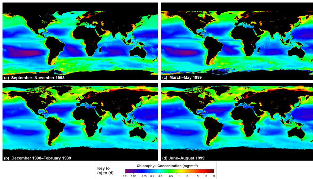
Figure 12-13. Seasonal variations in the distribution of chlorophyll in the surface waters of the world oceans for (a) September to November, (b) December to February, (c) March to May, and (d) June to August. Chlorophyll concentration is a reasonable measure of primary production. The data were obtained by a satellite sensor that measures ocean surface color within several wavelength bands. Black areas are land or where there were no data, because of cloud or ice cover or the limited orbital coverage of the satellite near the poles. Note the high productivity of many coastal regions and of the high-latitude seas in the Northern Hemisphere.
