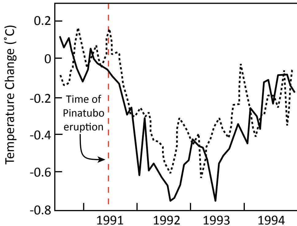
Figure 1.6B Comparison of predicted (solid line) and observed (dashed line) global tropospheric temperatures. [Hansen, J., et al. 1996. A Pinatubo climate modeling investigation. In The Mount Pinatubo Eruption: Effects on the Atmosphere and Climate. NATO ASI Series Vol. I 42, pp. 233-272. Springer-Verlag. Heidelberg, Germany]
