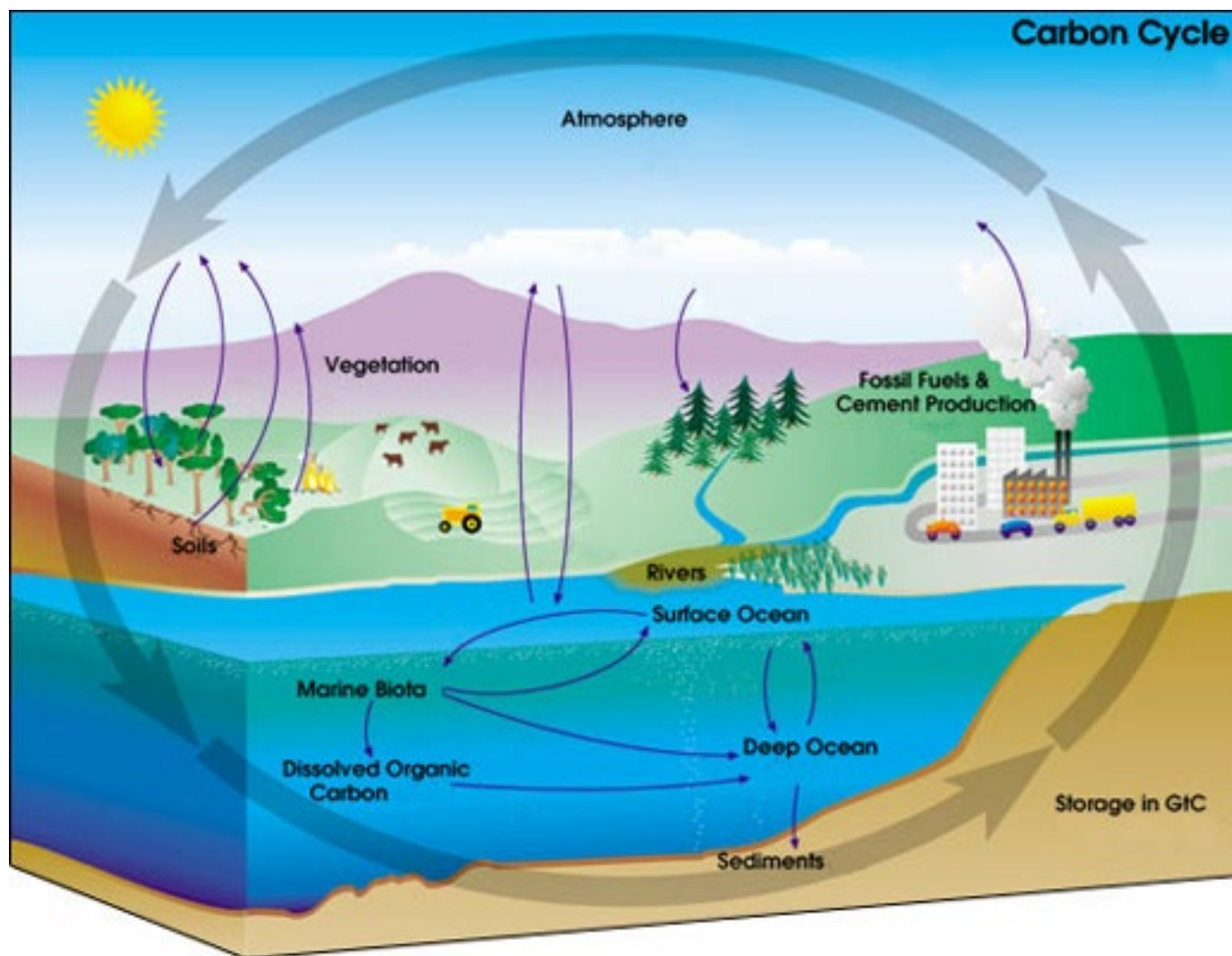
Figure 1.24 The carbon cycle. [NASA]
