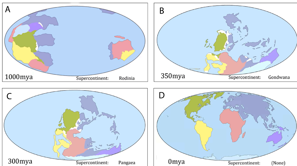
Figure 6. Supercontinents (A) Rodinia, (B) Gondwana, (C) Pangaea, and the (D) current continental configuration. [Modified from AlgolZ ]
