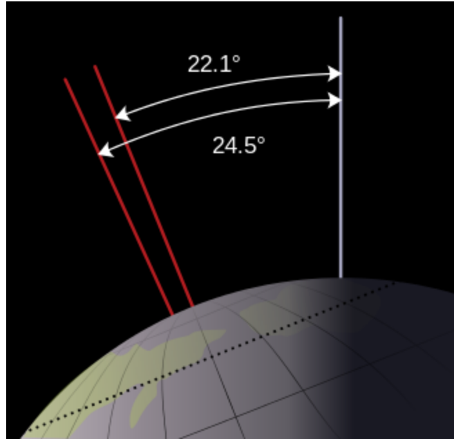
Figure 5. Earth's obliquity cycles from 22.1° to 24.5°. [ Energy Education ]
