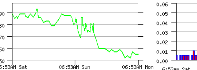
Portland, Portland International Airport - NWS/FAA Relative Humidity (percent)
