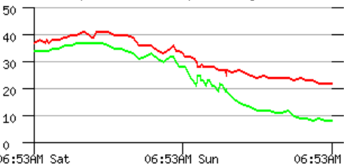
Portland, Portland International Airport - NWS/FAA Temperature and Dewpoint (Degrees F)
